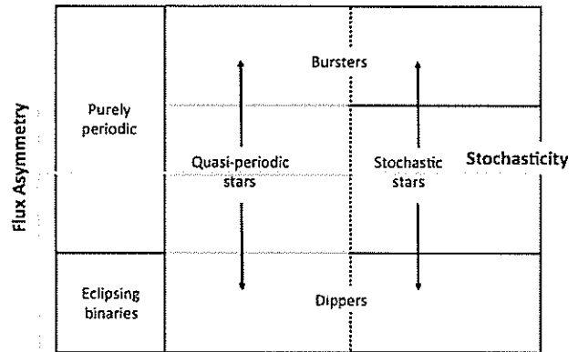
Figure 8. Schematic of the classification system we have applied for optical and infrared variability in the CSI 2264 data set. At the top end of the schematic are light curves preferentially populated with brightening events on top of a continuum, while at the bottom of the schematic are light curves with fading events. The middle is occupied by variability that is more or less symmetric in flux. Moving from right to left are variables with increasingly stable repeating patterns.
