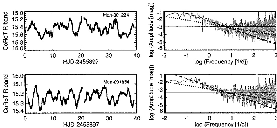
Figure 17. Light curves for two prototypical stochastically behaving stars, along with their Fourier transform periodograms, shown here in log space. Each Fourier transform consists of three parts: a relatively flat low-frequency regime, a steeper red noise trend from \log(f) \sim -1 to 1, and a flat white-noise-dominated regime for log frequencies beyond 1.0. We have fitted the white noise with a single value, shown as a black line. The red noise is modeled by a 1/\sqrt{f} trend in amplitude (i.e., 1/f in power; dashed line) and a 1/f trend in amplitude (dotted line), the latter of which fits the data much better.
