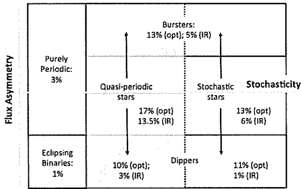
Figure 24. Schematic of the optical and infrared variability types detected in our 162 member disk-bearing data set, with optical (“opt”) and infrared (“IR”) fractions. Not noted here are the percentages of long-timescale and unclassifiable variables, as well as non-variables; hence, the listed values do not add up to 100%.
