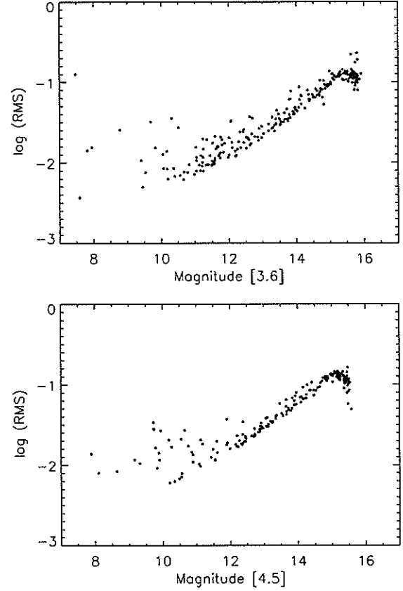
Figure 48. Standard deviations for the first section of IRAC staring light curves in channel 1 (top) and channel 2 (bottom), as a function of magnitude. The lower envelope of values closely matches the uncertainties predicted by Poisson noise and sky background, whereas the higher values are due to stellar variability.
