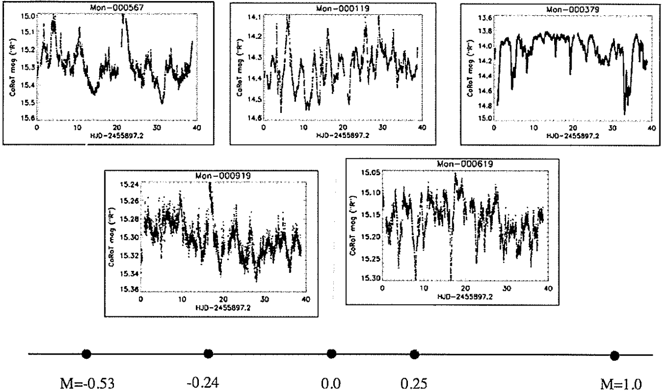
Figure 30. CoRoT light curves with representative values of the M parameter, ranging from bursting ( M < -0.25 ) to symmetric ( M = -0.25 – 0.25 ) to dipping ( M > 0.25 ).
