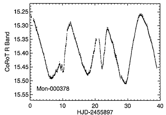
Figure 23. The unusual optical light curve of Mon-000378. This may be a combination of periodic behavior and circumstellar obscuration.
