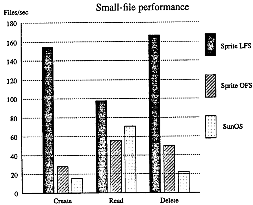
Figure 6-1 — Small-file performance
