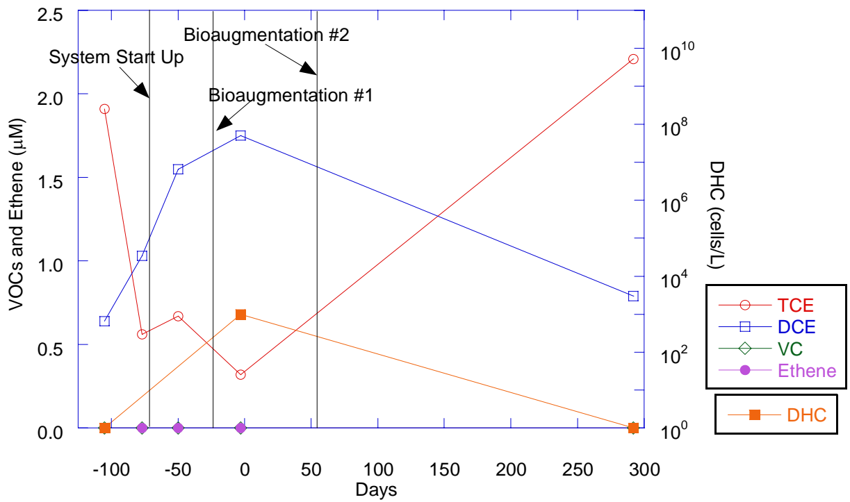
Figure I-10. Chlorinated Ethenes, Ethene, and DHC: Monitoring Well BMW-10 (Loop 1)
