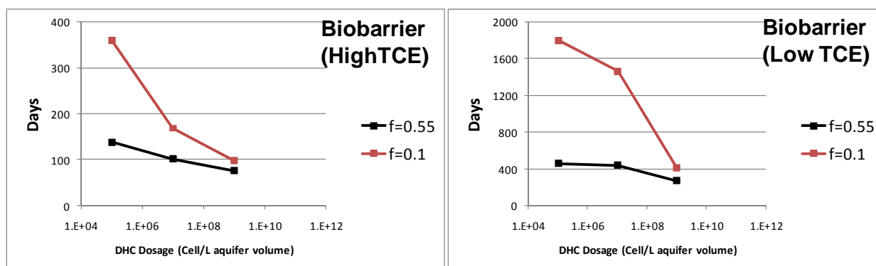
FIGURE 6-4. Model simulation of cell dosage effects on treatment of TCE in biobarrier applications (Schaefer et al., 2009). Data represent the amount of time required to reach 99% removal of cVOCs. All simulations assumed a groundwater velocity of 0.5 ft/day. High concentration TCE was 0.5 mM, and low concentration TCE was 0.005 mM.
