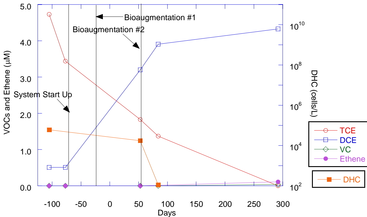
Figure I-15. Chlorinated Ethenes, Ethene, and DHC: Injection Well IW-1 (Loop 1)
