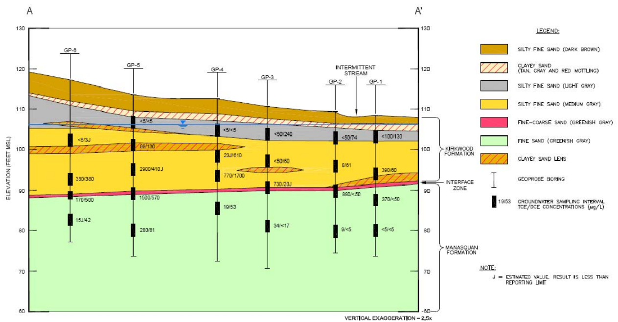
Figure 1. Demonstration area geologic cross-section and contaminant distribution.
