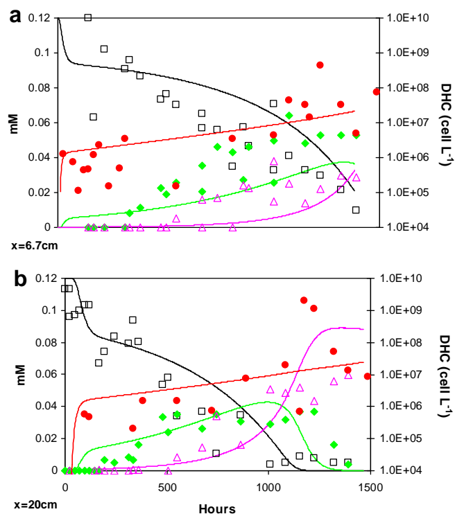
Fig. 6. Changes in chlorinated ethene and ethene concentrations (mM) and DHC concentration ( \text{cell L}^{-1} ) with respect to time during the column experiments at (a) 6.7 cm and (b) 20 cm from the influent. DCE - \square , VC - \blacklozenge , Ethene - \triangle , DHC - \bullet . Results from replicate columns are plotted. The corresponding lines represent model predictions using the dechlorination enhancement factor of 200 that was measured in the batch experiments performed on the column effluent.
