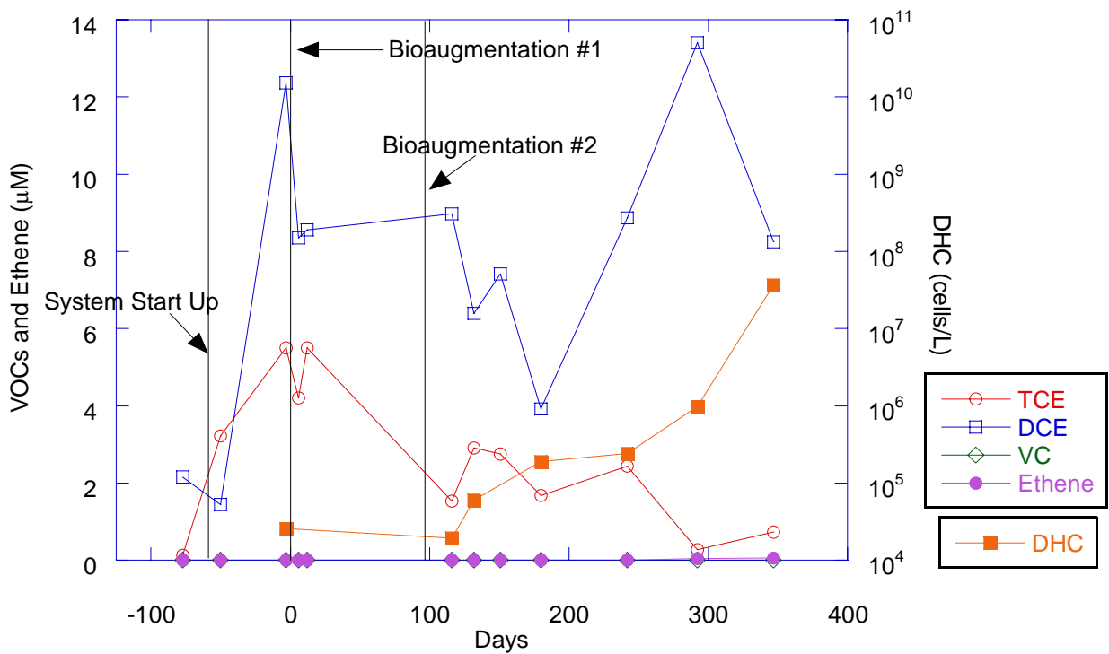
Figure I-20. Chlorinated Ethenes, Ethene, and DHC: Extraction Well EX-2 (Loop 2)
