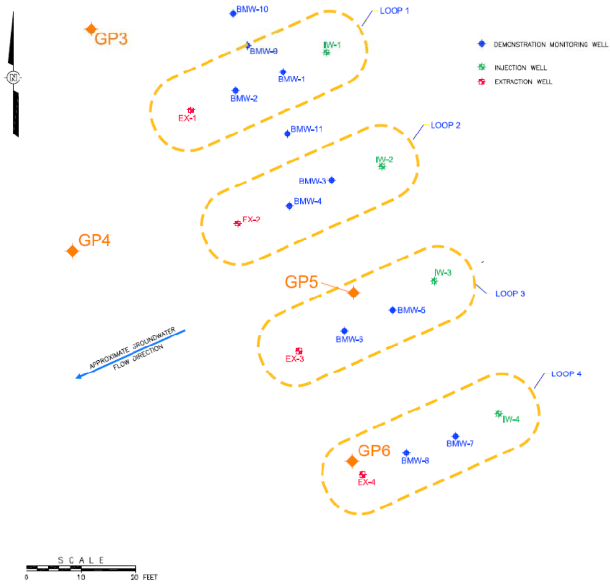
Figure 2. Demonstration layout.
