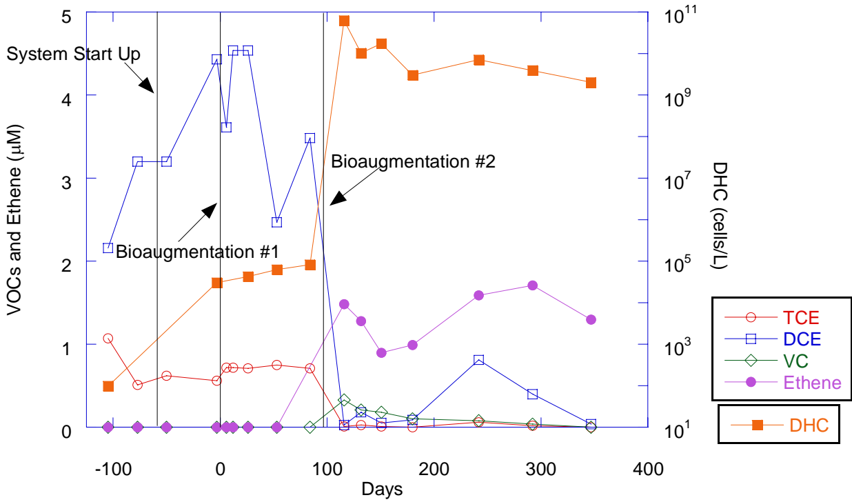
Figure I-1. Chlorinated Ethenes, Ethene, and DHC: Monitoring Well BMW-1 (Loop 1)
