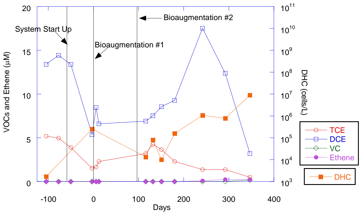
Figure I-4. Chlorinated Ethenes, Ethene, and DHC: Monitoring Well BMW-4 (Loop 2)
