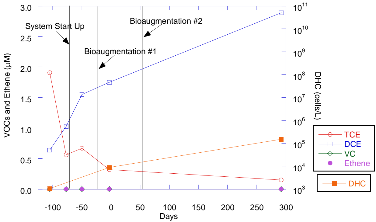
Figure I-9. Chlorinated Ethenes, Ethene, and DHC: Monitoring Well BMW-9 (Loop 1)
