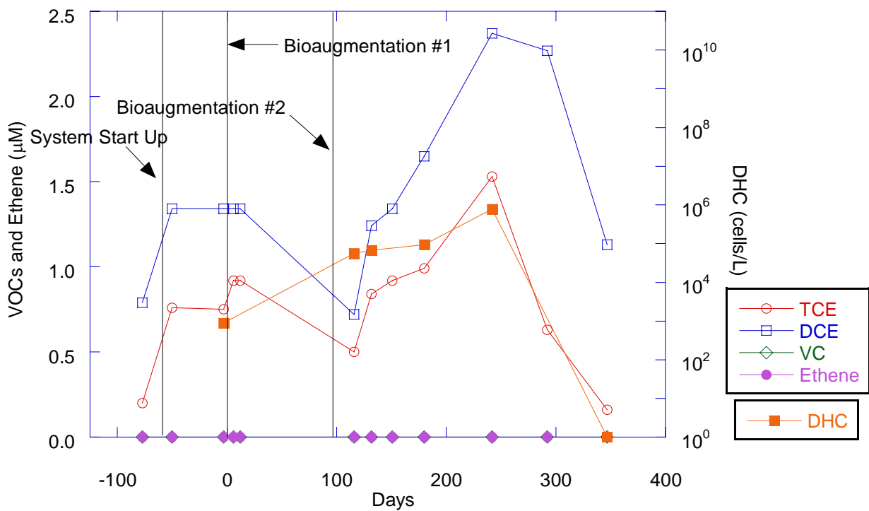
Figure I-22. Chlorinated Ethenes, Ethene, and DHC: Extraction Well EX-4 (Loop 4)
