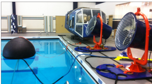
A wave generator and two high-speed fans, part of a suite of environmental condition simulation equipment installed by the Air Force in its water-egress training facilities. Special Operations Command (SOCOM) installed similar equipment in its facility. SOCOM officials said they used the equipment to increase the realism of their water-egress and water survival training. Air Force officials said the Air Force uses the equipment for the same purpose in its water survival training.
