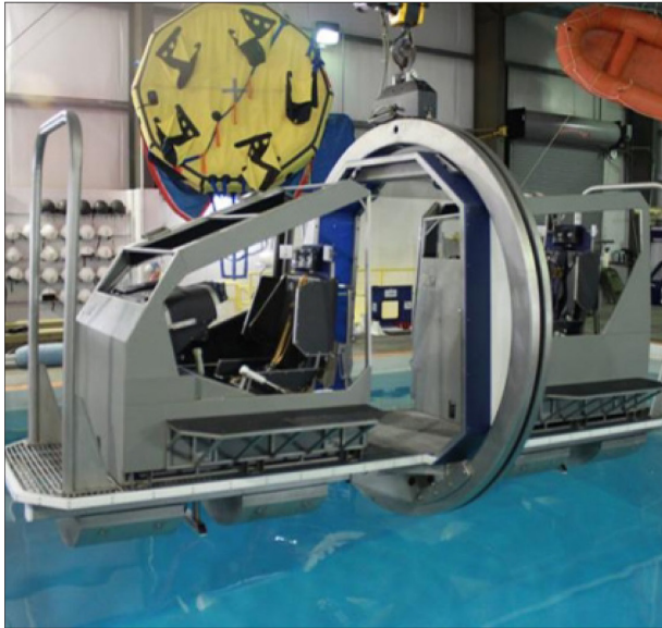
An AH-64 Apache Modular Egress Training Simulator, a type of egress simulator used by the Army to train its Apache pilots and aircrew on a replica of their specific airframe.
