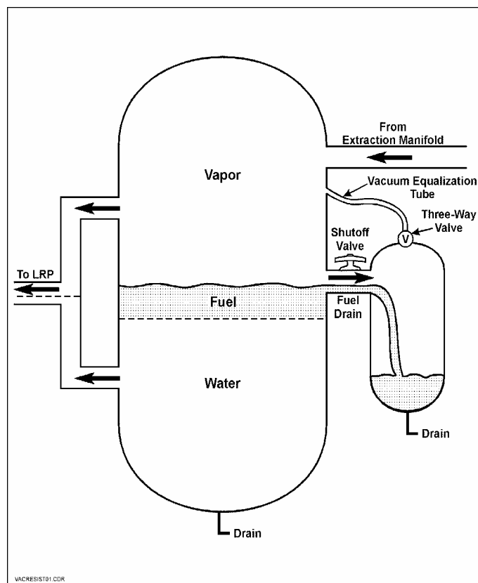
Figure 1. Vacuum-Resistant Separator.
