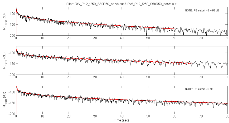
Figure 23. Reverberation Workshop Problem 12: PE method reverberation results for surface (top), volume (middle), and bottom reverberation at 250 Hz.
