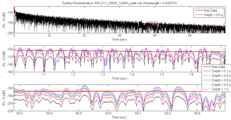
Figure 49. RW Problem 11 at 3500 Hz (isovelocity). Reverberation time series based on near surface transmission loss. Top plot shows full time series for using TL result at depth 0.6 \lambda ; middle plot shows near range reverberation time series detail for all near surface depths; bottom plot shows long range reverberation time series detail for all near surface depths.
