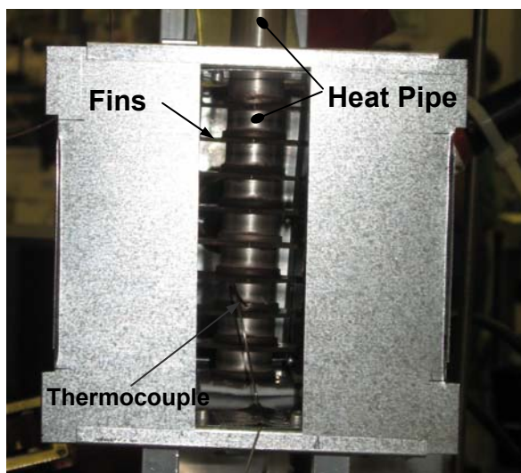
Figure 30 Duct Outlet View
