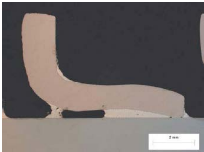
Figure 4 Fin Braze Detail from EWI Welding Report (N00014-02-C-0106)
