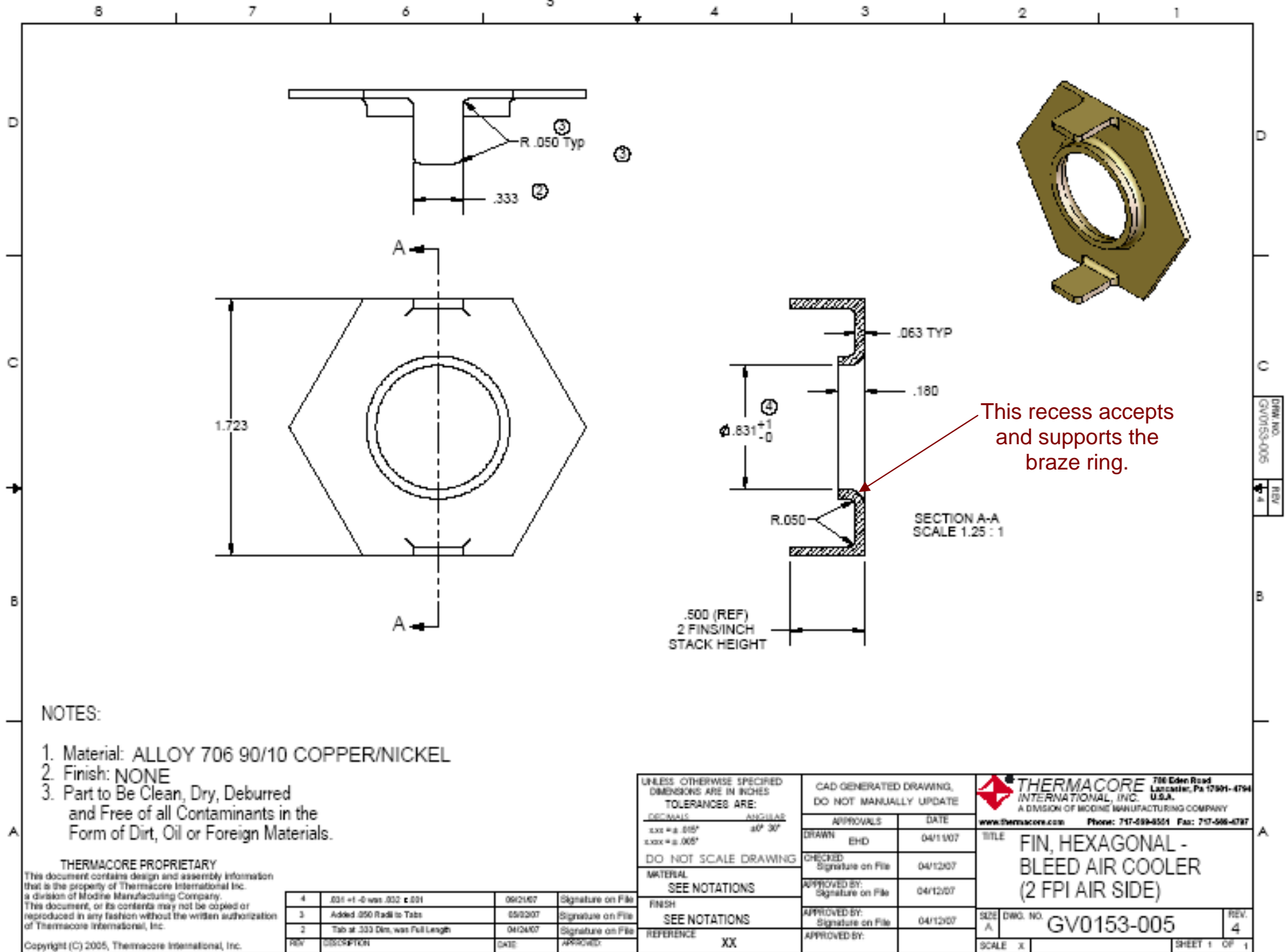
Figure 2 Design for Air Side Inlet Fin
