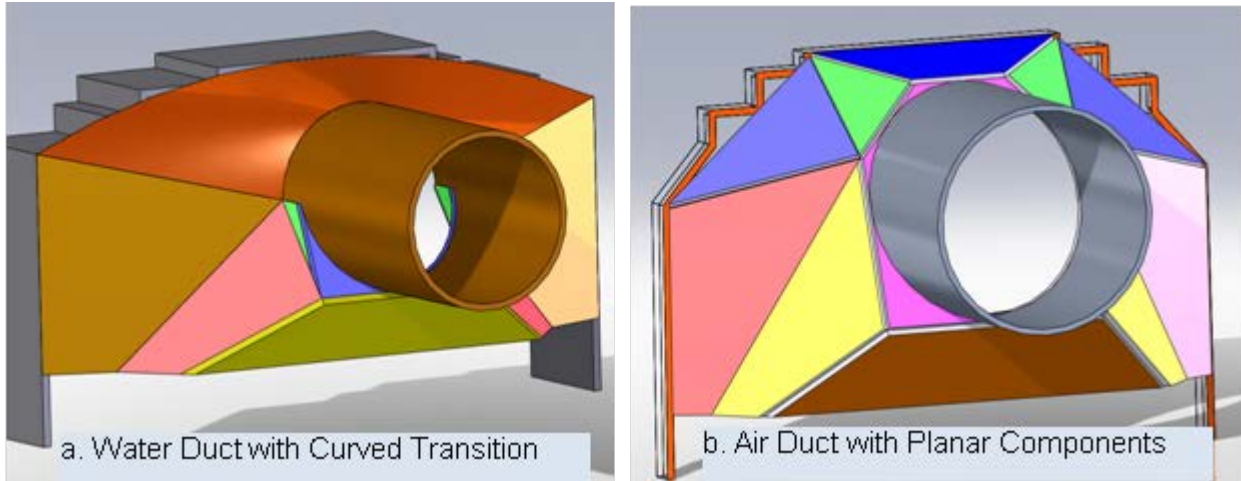
Figure 5- 4 Duct Designs
