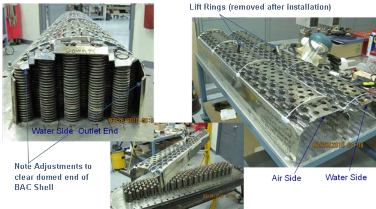
Figure 6- 1 Baffle Assemblies for Extended Length Heat Pipes, As-Built
