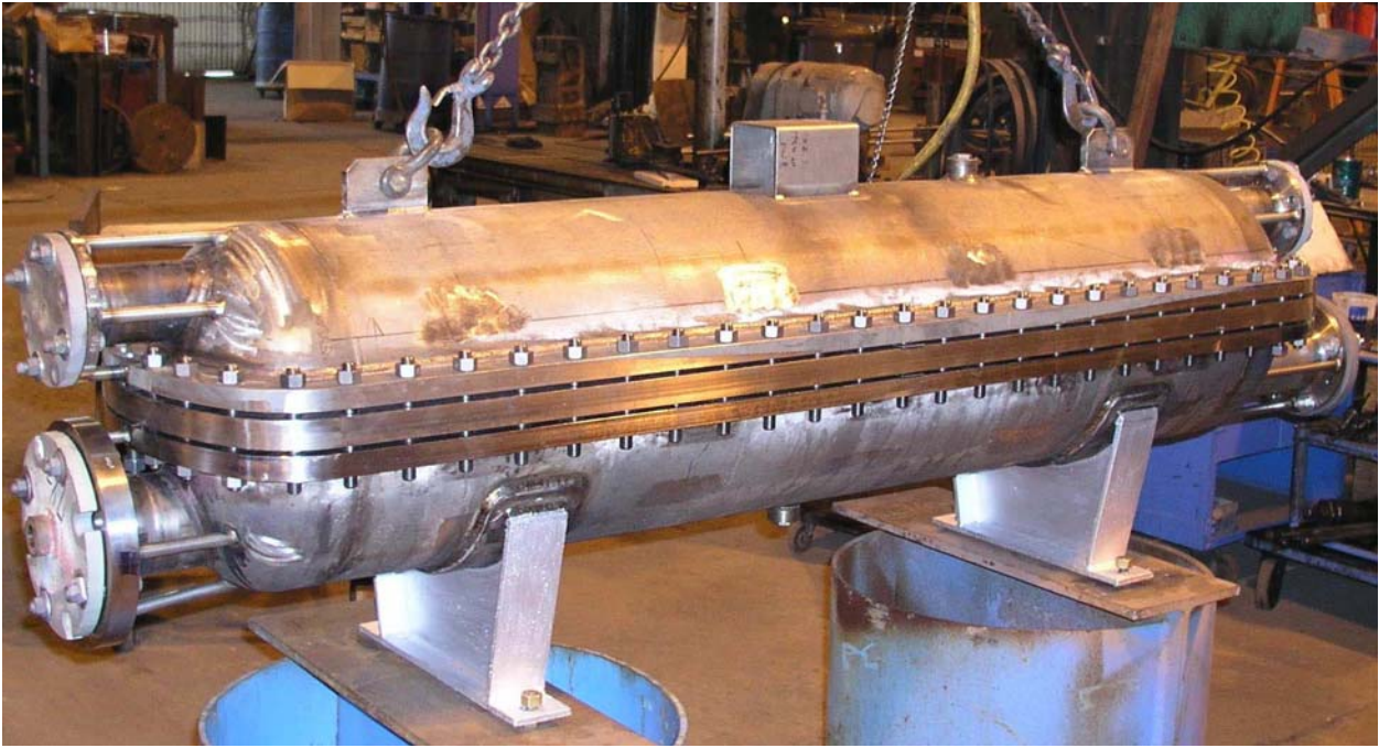
Figure 4 - BAC Assembly Step 2
