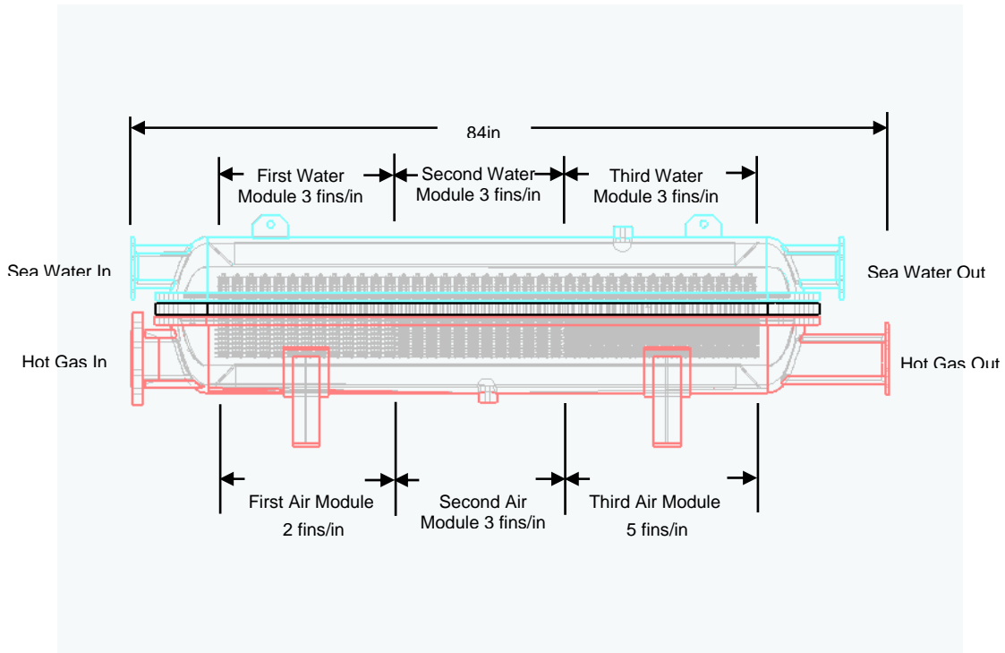
Figure 4. Side View illustrating the Three Heat Pipe Sections.
