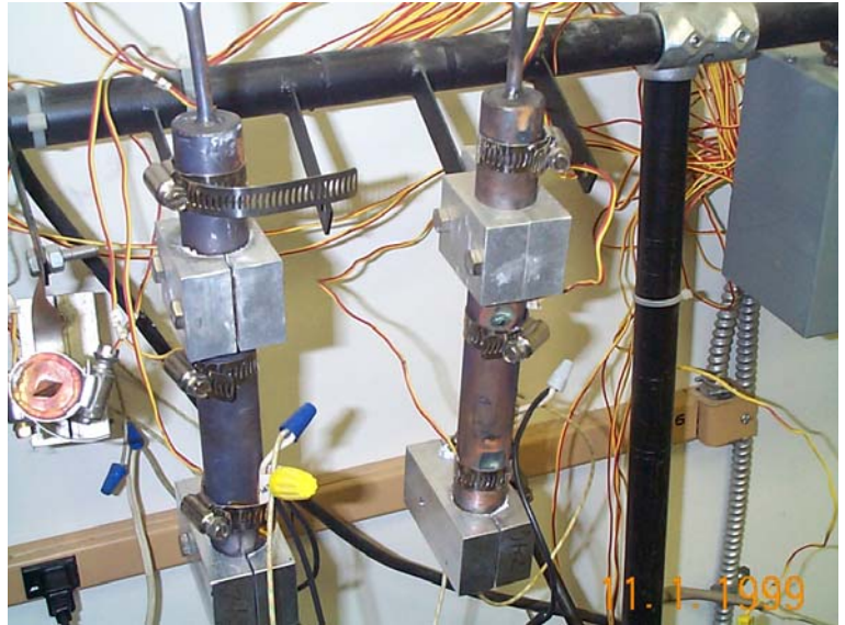
Figure C1. Pipes 745 and 746 on Life Test Rack
