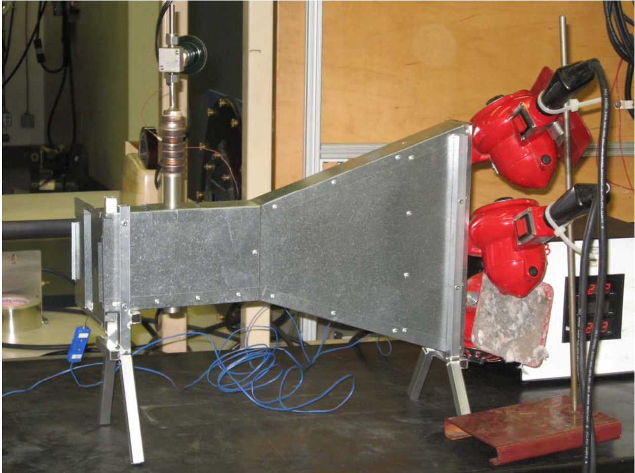
Figure 4 HP#1 in Test Duct
