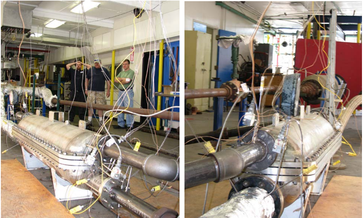
Bleed Air Cooler Engineering Unit on test at Wyle Laboratories, April 17, 2008
