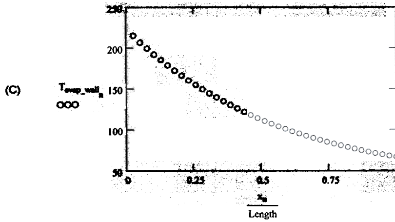
Heat Pipe Evaporator Wall Temperature vs. Normalized Exchanger Length
