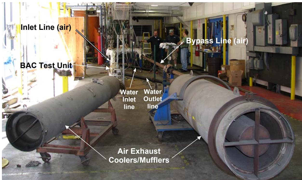
Figure 24 Setup at Wyle Labs Test Facility View from Air Exhaust Side
