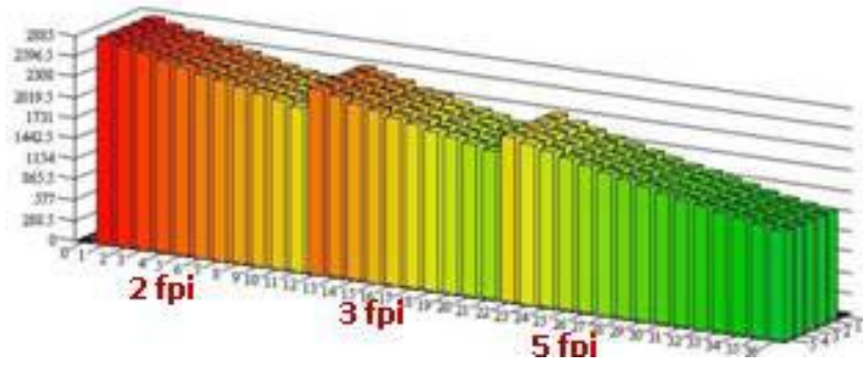
Figure 4- 3 Temperature and Power per HP
