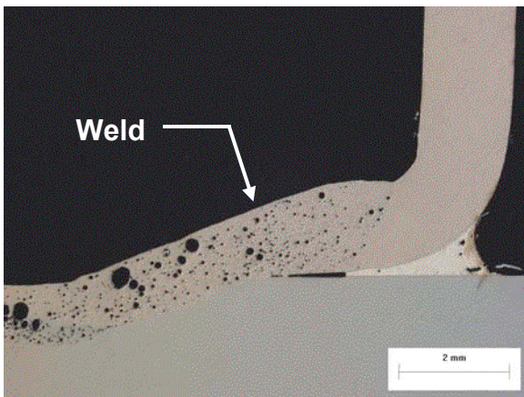
Figure 27 - Assembly #3 Braze Joint Voids with Porosity in Adjacent Weld
