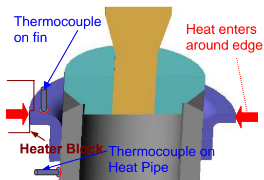
Figure 8 T/C's and Heat Input
