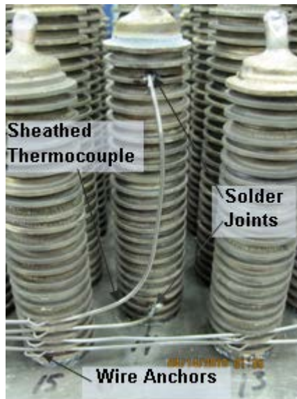
Figure 6- 8 Thermocouples
