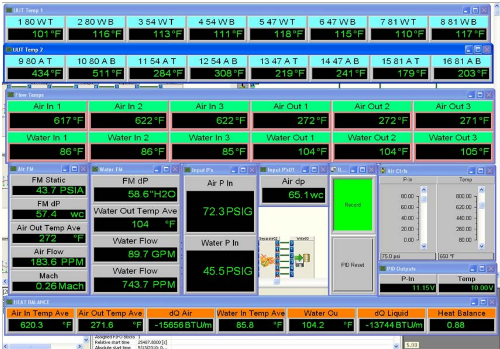
Figure 7- 7 Data Set 3 at 620 ° F (5:51 PM 5/13/10)
