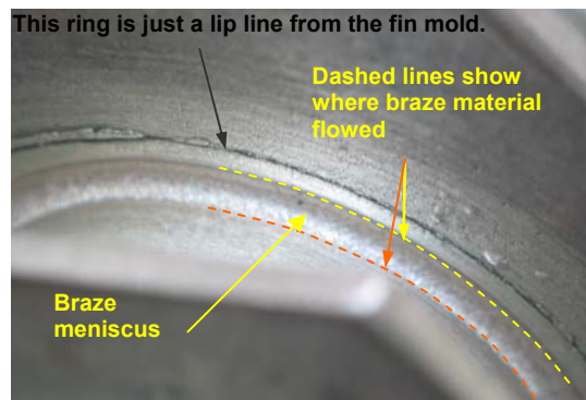
Figure 6 Close-up View of Braze
