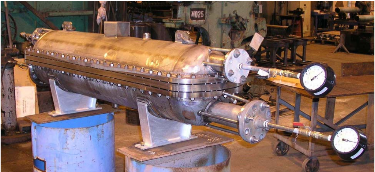
Figure 5 - BAC Assembly Step 3
