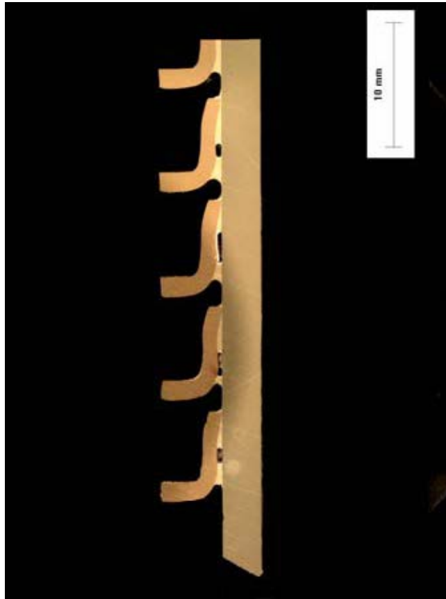
Figure 3- 8 Original Fin Braze
