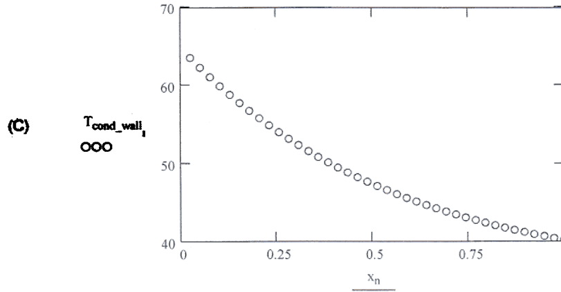
Heat Pipe Condenser Wall Temperature vs. Normalized Exchanger Length
