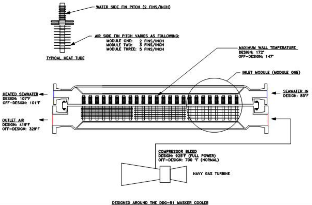
Figure 2-3 Proposed Full Scale "Heat Pipe" Heat Exchanger
