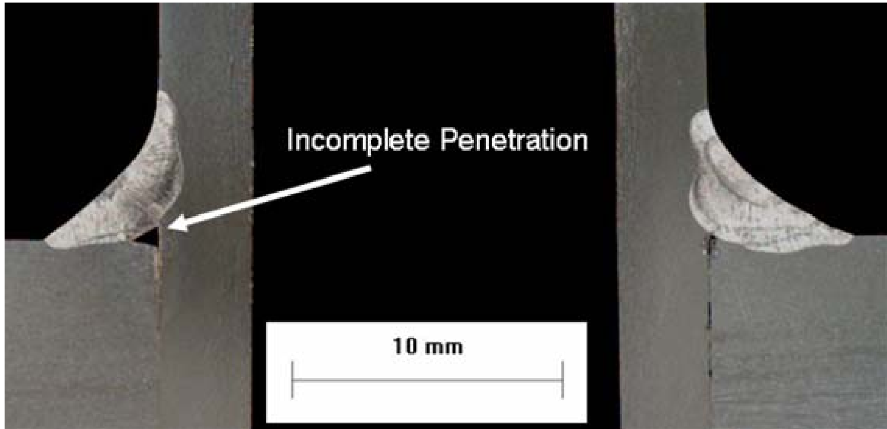
Figure 18 - Cross Section of EWJ Consumable Insert Weld
