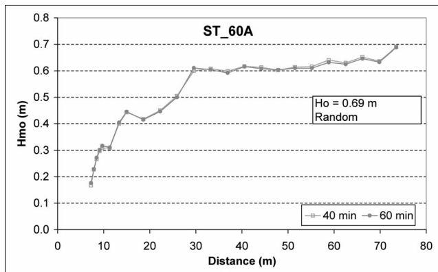
Figure 10. Cross-shore wave-height distribution measured during SUPERTANK ST.60A.
