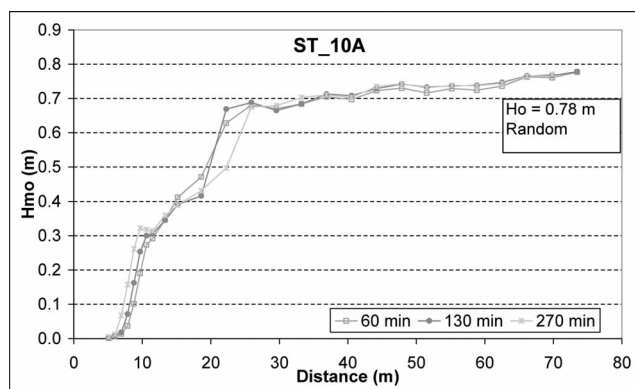
Figure 8. Cross-shore wave-height distribution measured during SUPERTANK ST.10A.
