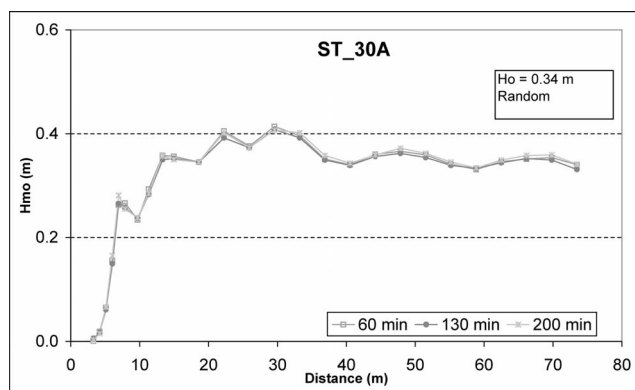
Figure 9. Cross-shore wave-height distribution measured during SUPERTANK ST.30A.
