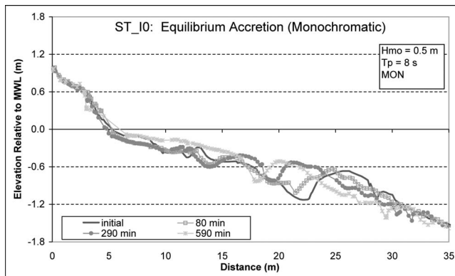
Figure 5. The SUPERTANK ST_I0 accretionary monochromatic wave run. The resulting beach profile under monochromatic waves is erratic and undulating.
