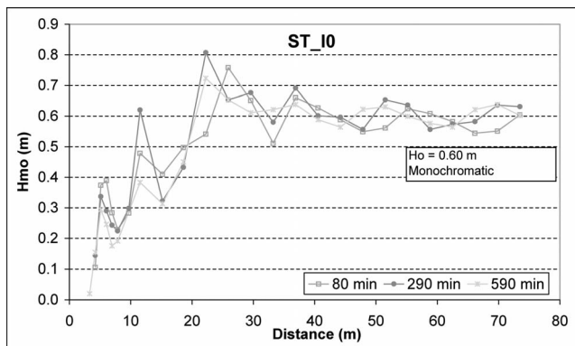
Figure 11. Cross-shore wave-height distribution measured during SUPERTANK ST.10.
