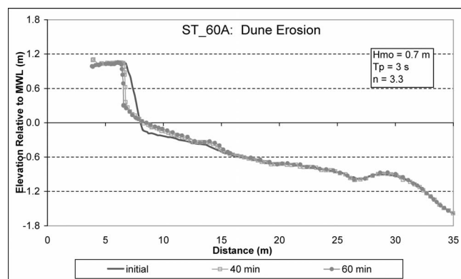
Figure 4. The SUPERTANK ST_60A dune erosion wave run. A nearly vertical scarp developed after 40 min of wave action, with the upper limit of beach change identified at the toe of the dune scarp.
