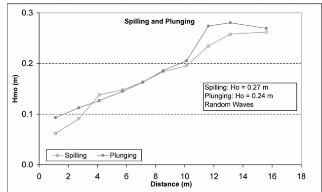
Figure 12. Cross-shore wave-height distribution for the LSTF spilling and plunging wave cases.
