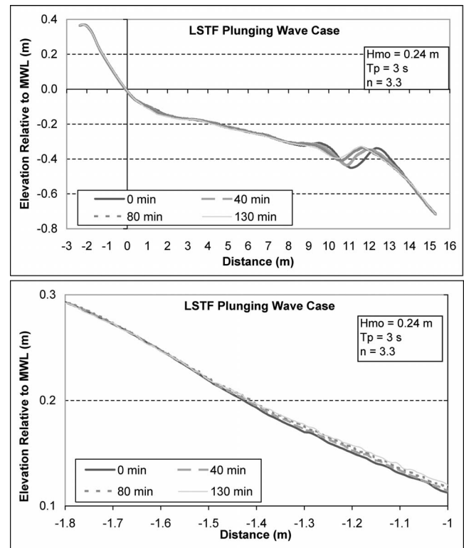
Figure 7. The LSTF plunging wave case. Slight foreshore accretion and landward migration of the offshore bar occurred during the wave run.
