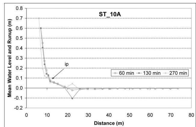
Figure 13. Wave runup measured during SUPERTANK ST.10A. The arrow with notation "ip" refers to the inflection point between the wave setup and runup.
