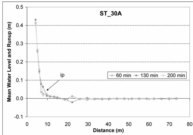
Figure 14. Wave runup measured during SUPERTANK ST.30A. The arrow with notation “ip” refers to the inflection point between the wave setup and runup.
