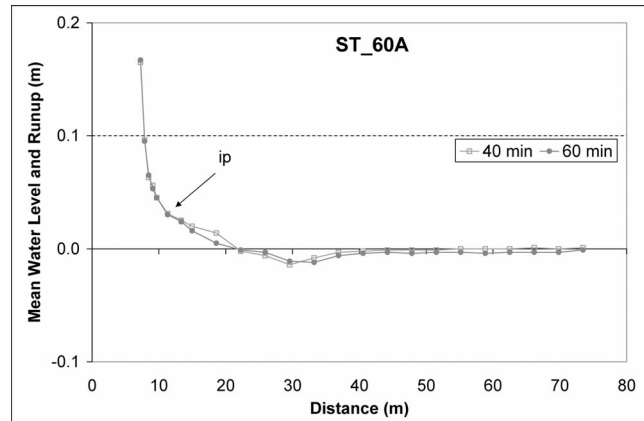
Figure 15. Wave runup measured during SUPERTANK ST.60A. The arrow with notation “ip” refers to the inflection point between the wave setup and runup.
