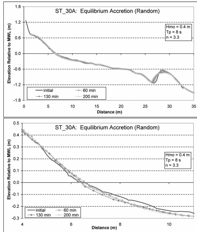
Figure 3. The SUPERTANK ST_30A accretionary wave run. There was subtle beach-face accretion, with an onshore migration of the offshore bar (top). The accretion near the shoreline is identified if viewed at local scale (bottom).
