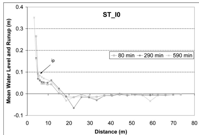
Figure 16. Wave runup measured during SUPERTANK ST.I0. The arrow with notation “ip” refers to the inflection point between the wave setup and runup.
