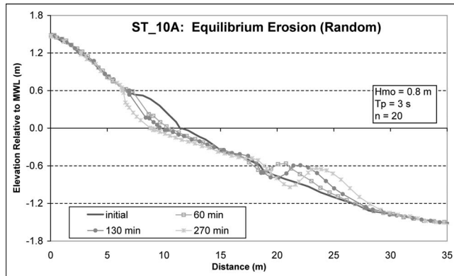
Figure 2. The first SUPERTANK wave run, ST_10A erosional case. Substantial shoreline erosion occurred on the initial monotonic profile with the development of an offshore bar. The horizontal axis “distance” refers to the SUPERTANK coordinate system and is not directly related to morphological features.
