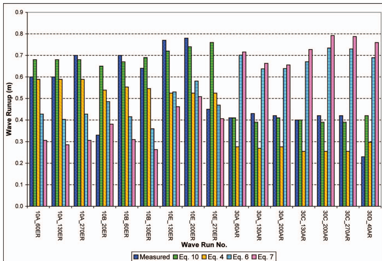
Figure 18. Comparison of measured and predicted wave runup.
