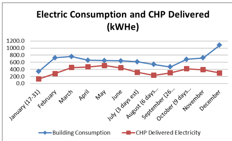
Figure 11. Monthly electrical consumption and production.
