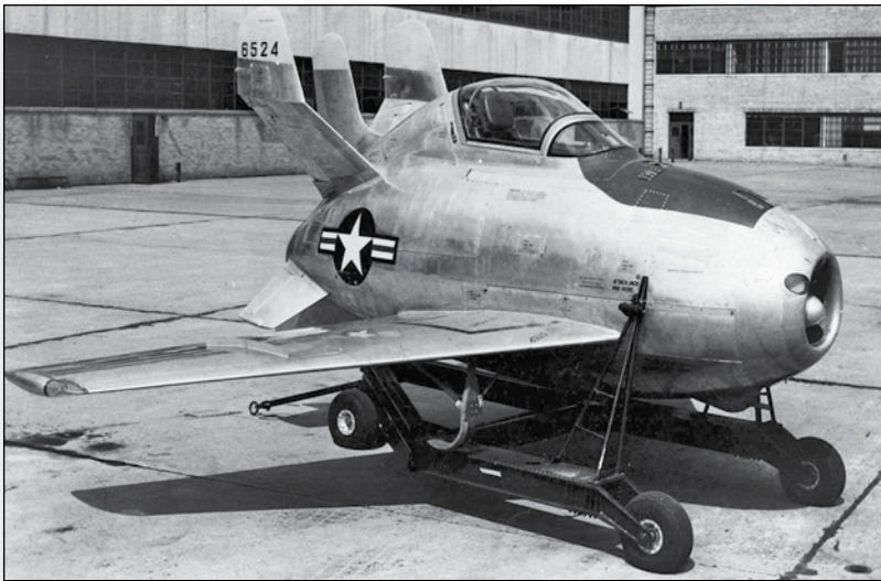
The McDonnell XF-85 Goblin, the smallest jet fighter ever built, was designed to fit entirely inside the bomb bay of a B-36, allowing the heavy bomber to carry its own fighter escort.
