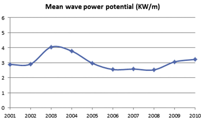
Fig. 17. Yearly mean wave power potential for the area of Paphos.
