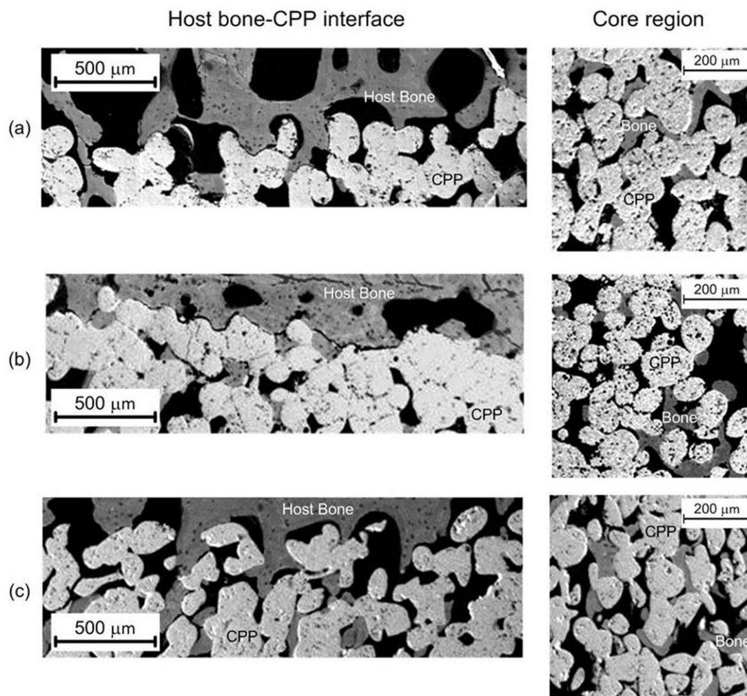
FIGURE 5. BSE images showing (right) bone formation in core region of implants and (left) the integration of CPP constructs and host bone in the interface of (a) SFF-V, (b) SFF-H, and (c) CS implants and surrounding bone. Qualitatively significant bone ingrowth within the different regions of the implants, including the central core regions and toward the circumferential regions nearest the host bone junction was observed. Bone ingrowth appeared uniformly distributed throughout the implants.
