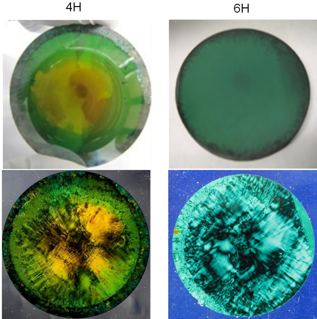
Figure 1. Optical and crossed polarizers images of the 4H and 6H SiC crystals. The top images are the optical images while the bottom images are from cross polarizers lighting.
