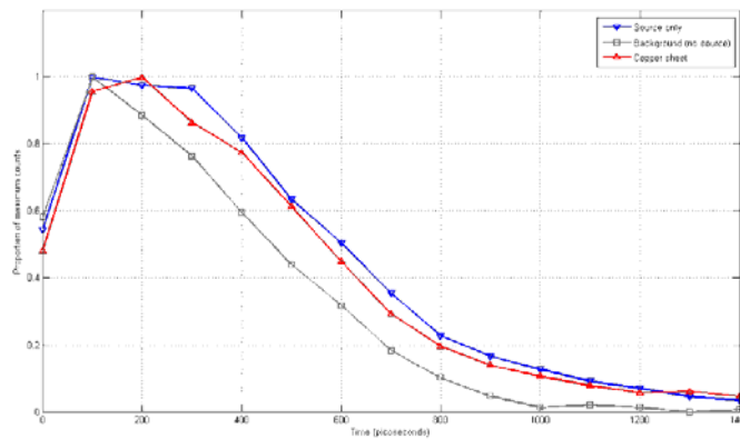
Figure 16: Lifetime spectra taken with no sample on the stage and with the copper plate sample present. These spectra will act as upper and lower bounds for the crystal spectra.
