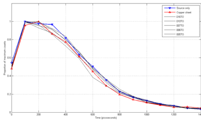
Figure 26: Collected spectra for all \text{ThO}_2 crystal samples.
