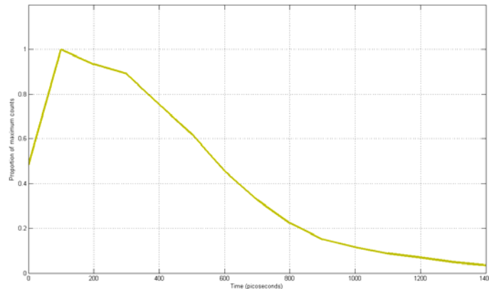
Figure 13: A representative PALS spectrum taken with a TAC/MCA system. Note the extremely fine binning of tens of picoseconds. [7]
