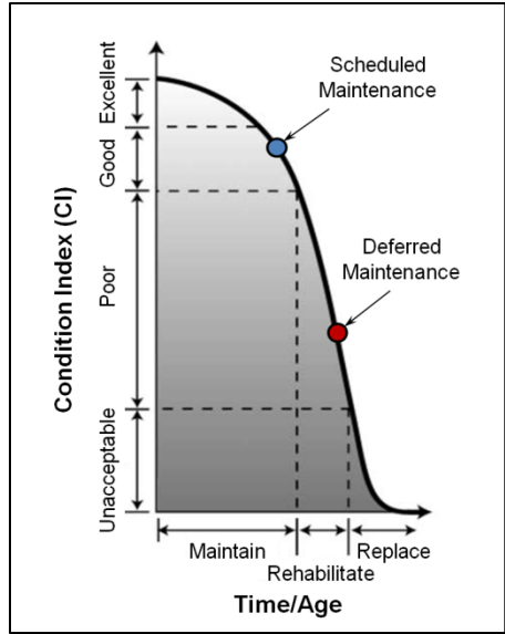
Figure 1. Component Degradation Curve (Dornan, 2002)
