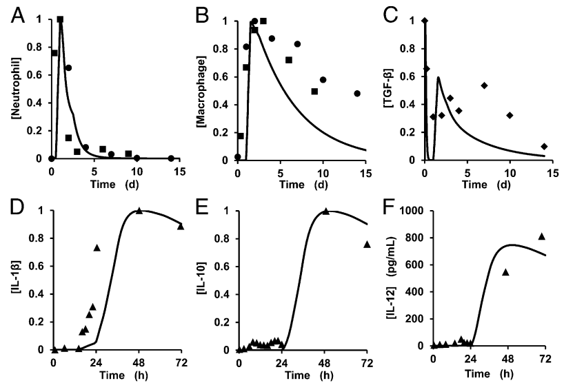
FIGURE 3. Modeling predictions capture experimentally detected kinetics of acute inflammation. Solid lines show modeling predictions; symbols show experimental data. Brackets designate concentration. (A–C) Experimental data for mouse infection (■) (16), rat wounds (◆) (53), and human wounds (●) (52). (D and E) Normalized values of IL-1 \beta and IL-10 concentrations in vitro. Experimental data from cultured human macrophages are shown (▲) (54). For proper comparisons between model predictions and experimental data, normalization was necessary because of differences in reporting units between experimental data and model outputs and was achieved by division of all of the predicted or experimentally obtained values of a particular variable by the maximum value of that variable. (F) IL-12 concentration dynamics in vitro. Experimental data were taken from Kum et al. (54).
