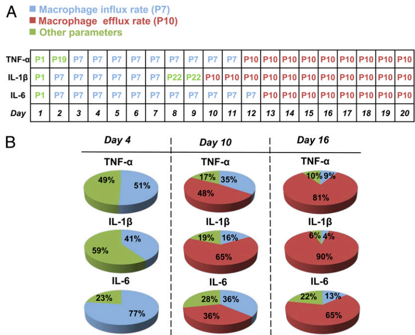
FIGURE 4. Sensitivity analysis identifies strong triggers of chronic inflammation. (A) Parameters inducing the largest changes in TNF- \alpha , IL-1 \beta , and IL-6 concentrations identified by local sensitivity analysis in the vicinity of the default parameter set (see Materials and Methods ). (B) Summary of local sensitivity analysis results for 10,000 randomly selected parameter sets (see Materials and Methods ) for three representative days (4, 10, and 16). Shown is the percentage of the 10,000 simulations for which the macrophage influx (blue) and efflux (red) parameters [identified in the analysis in (A)] induced the largest changes in TNF- \alpha , IL-1 \beta , and IL-6.
