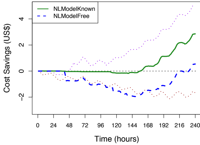
Figure 6.3: Cumulative cost savings over one episode for NLModelKnown and NLModelFree agent configurations.
