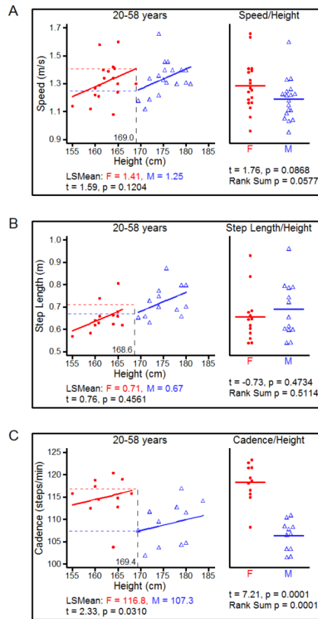
Figure 2: Plots of Height and Spatiotemporal Variables
