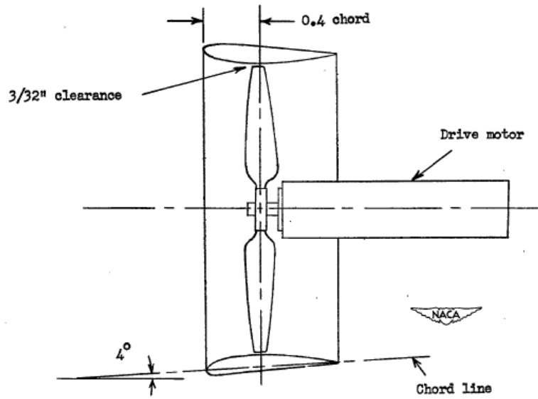
Figure 1.20: Hubbard's test arrangement [119].
