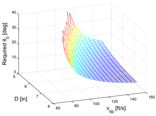
(b) Required collective
