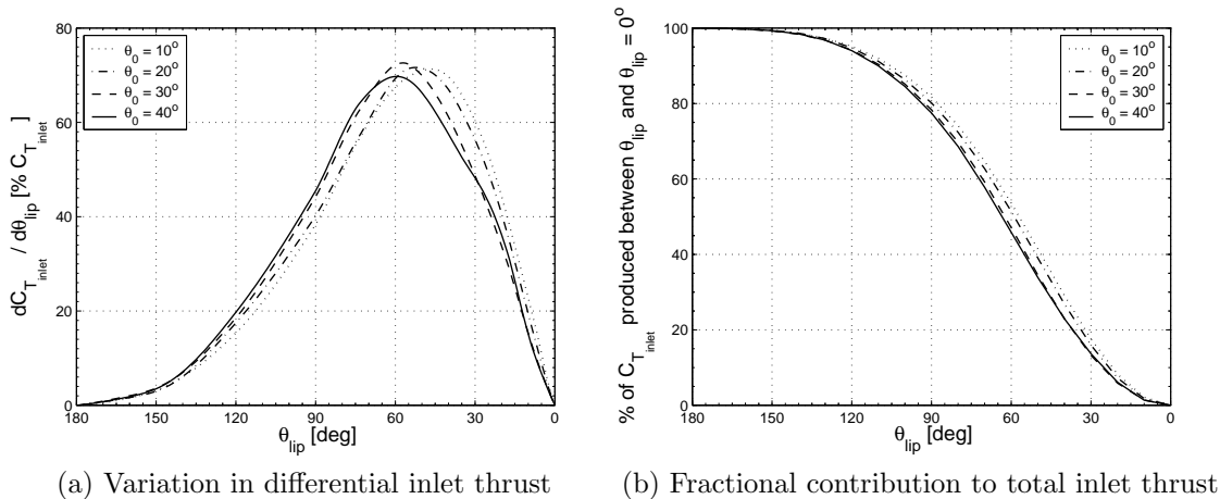
Figure 3.25: Inlet thrust distributions for model LR13-D10- \delta 0.1
