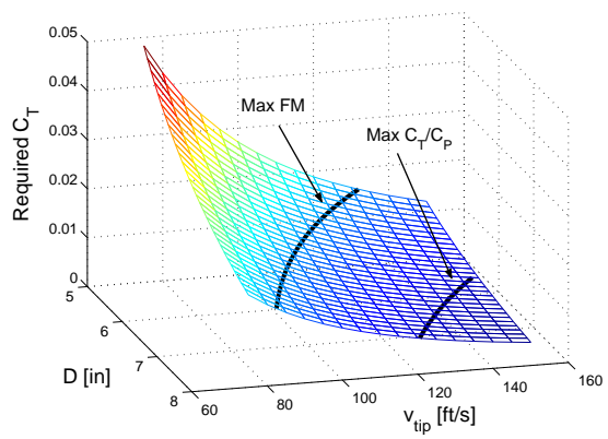
(c) Required thrust coefficient
