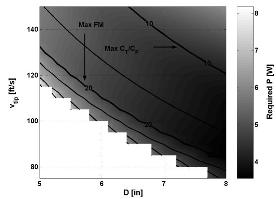
(e) Required power
