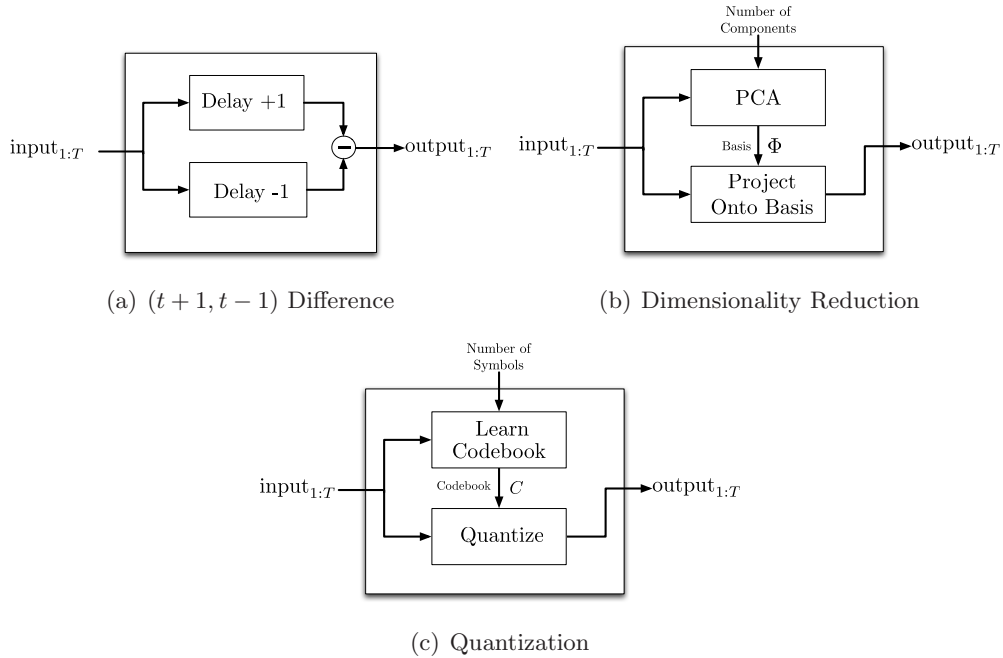
Figure 5.5. Sub-blocks for Audio and Video Processing: (a) A diagram showing how the (t+1, t-1) sub-block works. It outputs the difference between a positive and negative temporal delay of its input. (b) A diagram showing how dimensionality reduction is performed. Treating each sample independently PCA is performed on all of the input data to learn a basis \Phi with a specified number of components. All the data is then projected onto this basis. (c) A diagram showing how vector quantization is performed. All the data input data is used to learn a codebook with a specified number of symbols. We form this codebook by learning a Gaussian mixture model. The data is then quantized using this codebook, encoding each sample with the index of the mixture component best describes the sample.
