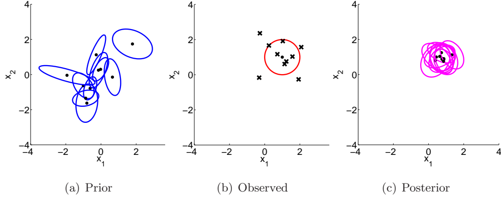
Figure 2.6. Examples of the Normal-Inverse-Wishart distribution: (a) Shows 10 2-d normal distributions with their parameters samples from a normal-inverse-wishart prior \mathcal{N}(\mu; \mathbf{0}, 2\Lambda) \mathcal{IW}(\Lambda; \mathbf{I}_2, 5) . Black dots represent the mean and the covariance is plotted as an ellipse. (b) Samples from a normal distribution with mean [1 \ 1]^\top and covariance \mathbf{I}_2 . (c) Gaussians with their parameters sampled from the posterior on parameters given the samples in (b).
