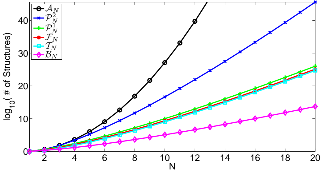
Figure 3.4. The Size of Sets of Directed Structure vs N: The number of possible structures as a function of N for the set of all directed structures \mathcal{A}_N , directed structures with at most 2, \mathcal{P}_N^2 , and 1, \mathcal{P}_N^1 parents, directed forests \mathcal{F}_N , directed trees \mathcal{T}_N , and factorizations \mathcal{B}_N .
