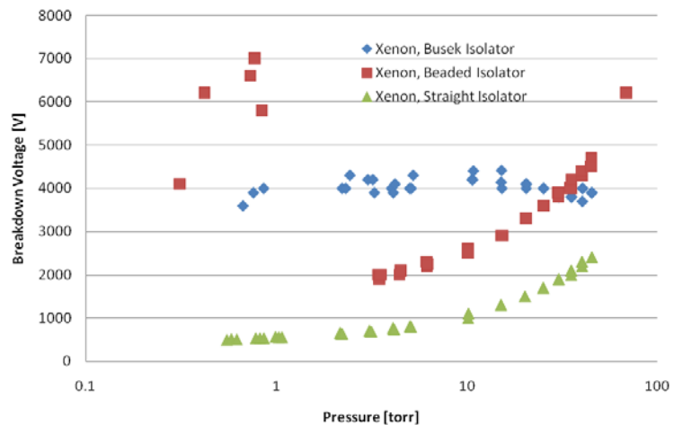
Figure 8. Breakdown voltage for xenon.
