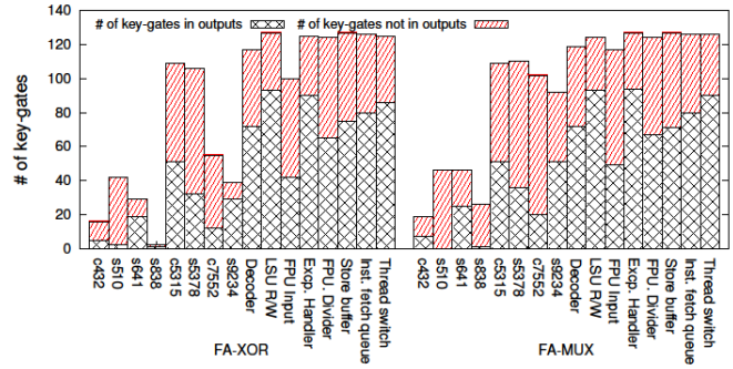
Figure 10. Number of key-gates inserted at the outputs and inside the designs for different fault analysis-based insertion techniques.
