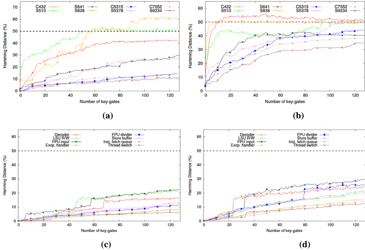
Figure 8. Hamming distance between the outputs of designs on applying the correct key and a random invalid key: (a) Random insertion of MUXes in ISCAS designs, (b) fault analysis-based insertion of MUXes in ISCAS designs, (c) random insertion of MUXes in OpenSPARC units, and (d) fault analysis-based insertion of MUXes in OpenSPARC units.
