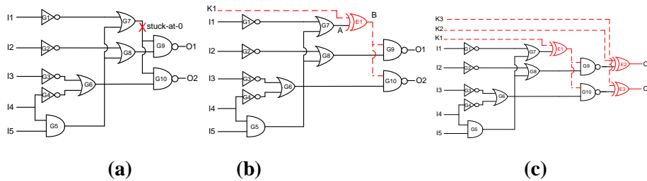
Figure 5. Relation between logic encryption and IC testing – (a) fault excitation, (b) propagation, and (c) masking.
