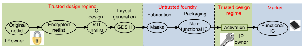
Figure 1. An IC design flow enhanced with logic encryption capabilities to thwart IC piracy [6,7]. Before sending the design to an untrusted foundry, the designer encrypts the design using logic encryption techniques. The foundry then manufactures this encrypted design. On receiving the encrypted hardware, the IC designer activates it by applying the secret key and the IC is then sold in the market.
