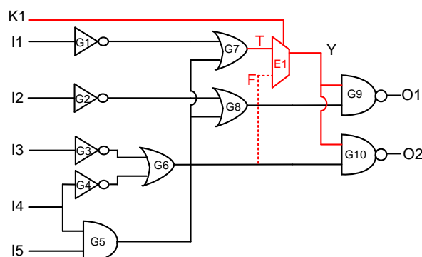
Figure 6. A circuit encrypted with one multiplexer (E1).
