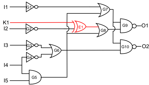
Figure 4. A circuit encrypted with one XOR-gate (E1). The valid key is K1=0.
