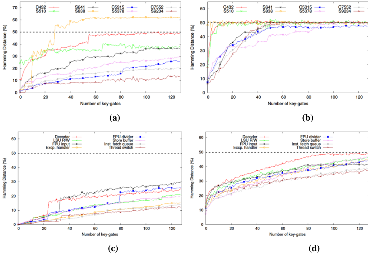
Figure 7. Hamming distance between the outputs of designs on applying the correct key and a random wrong key: (a) Random insertion of XORs in ISCAS designs [6,7,11], (b) fault analysis-based insertion of XORs in ISCAS designs, (c) random insertion of XORs in OpenSPARC [6,7,11], and (d) fault analysis-based insertion of XORs in OpenSPARC units.
