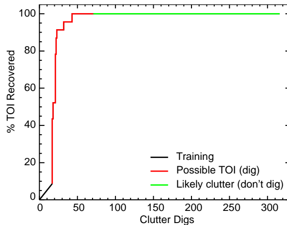
Figure 7-2 – TEMTADS MP 2x2 Cart Dynamic / Cued Classification Results for the former Spencer Artillery Range, TN. Classification performed by SAIC.
