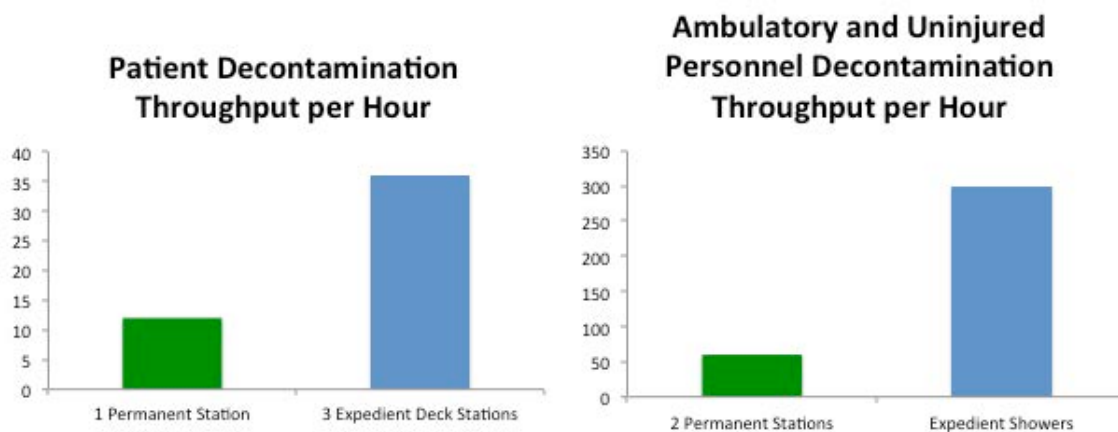
Figure 4.3 Increase in Decontamination Throughput with Expedient Deck Patient Decontamination Stations and Decontamination Showers
