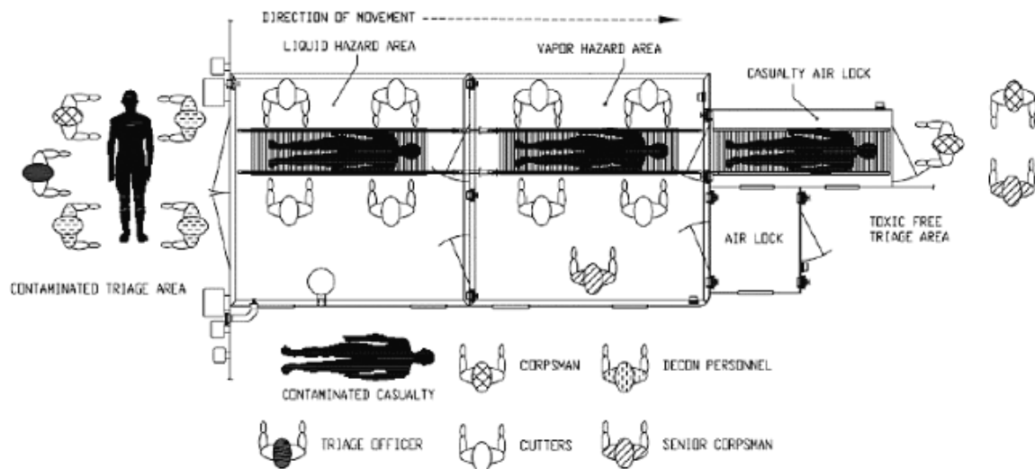
Figure 2.4 Patient Decontamination Station 15
