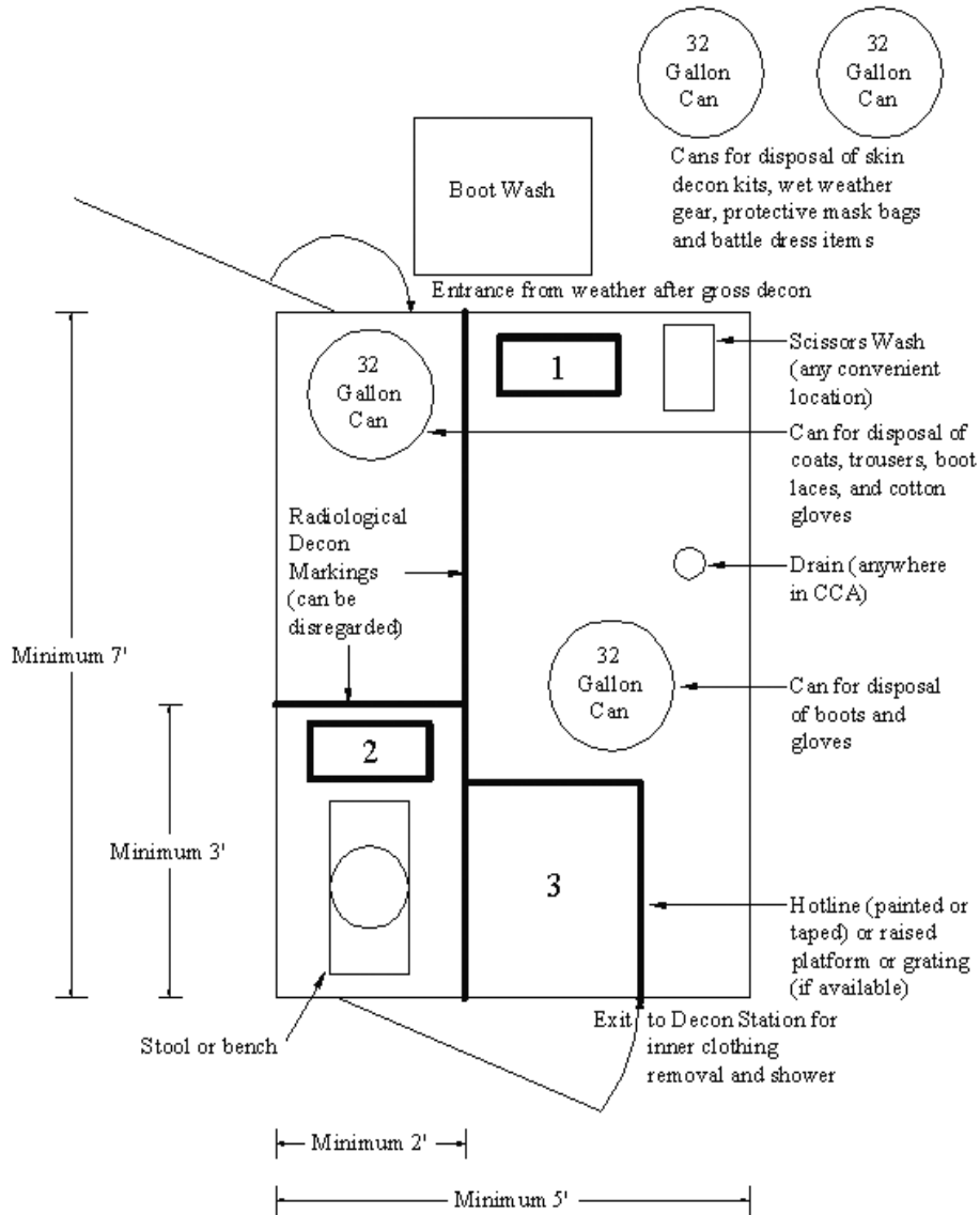
Figure 2.2 Contamination Control Area for Decontamination Step 1 13
