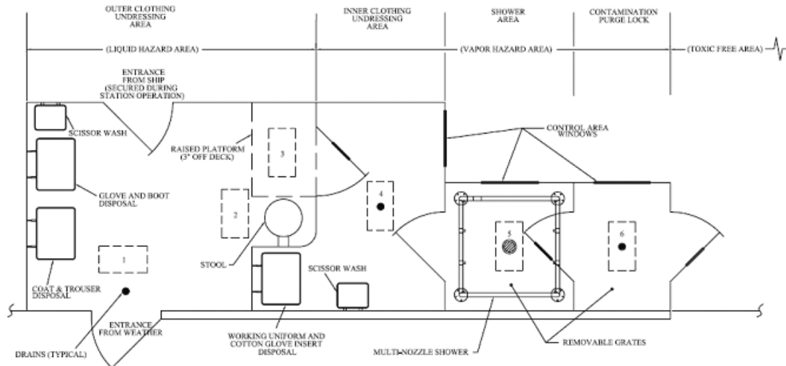
Figure 2.3 Contamination Control Area for Decontamination Steps 2-5 14
