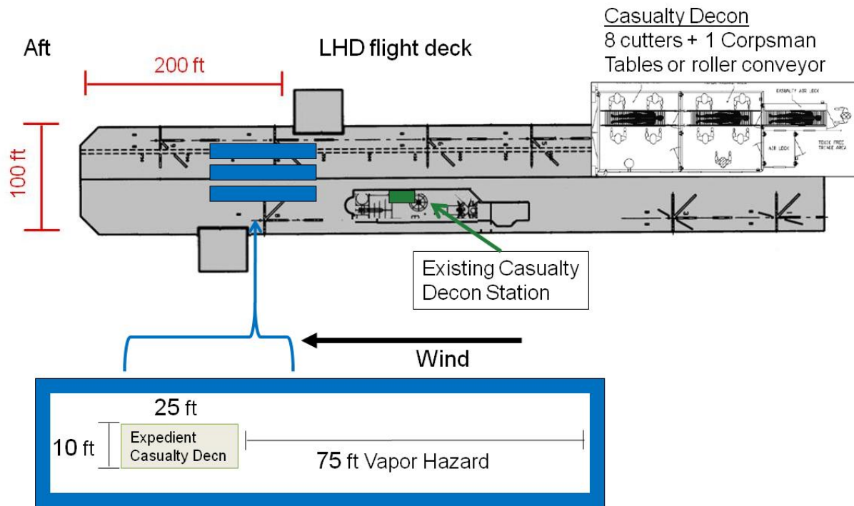
Figure 4.2 Expeditionary Patient Decontamination Stations on a LHD
