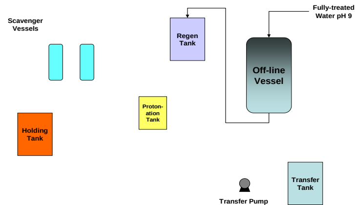
Figure 5-2. Regeneration Steps
