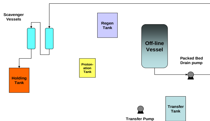
Figure 5-2. Regeneration Steps
