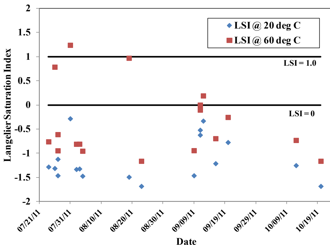
Figure 5-9. Langelier Saturation Index Results of WBA IX Treated Water For Test Periods 1-4
