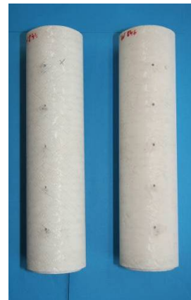
Figure 59: WHIPOX liners manufactured by DLR for transpiration cooling tests at TUM
