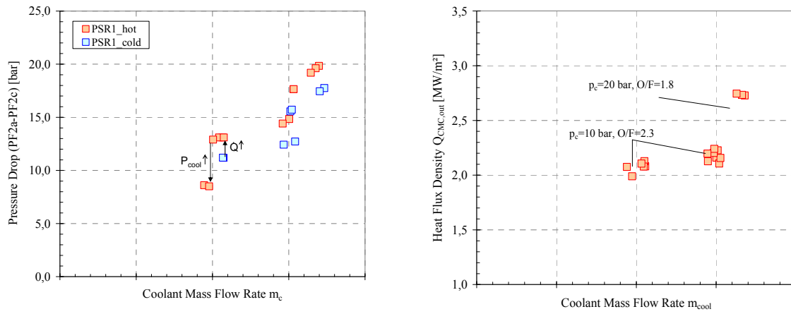
Figure 62: Pressure Drop and Heat flux evolution for Carbotex SI PSR
