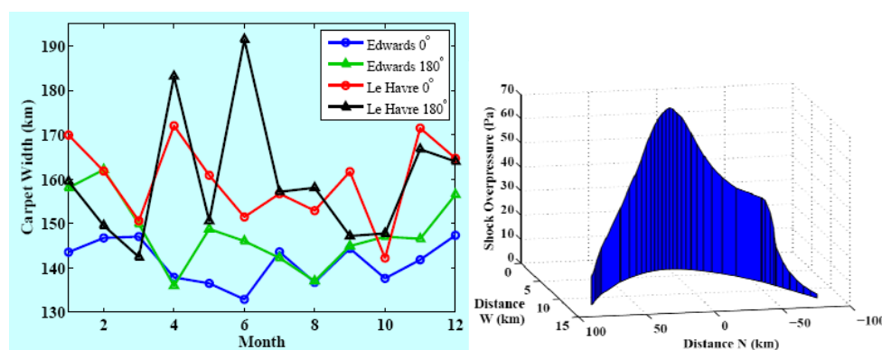
Figure 49: Sonic boom prediction for the Mach 6 reference configuration. Left : Carpet width prediction for two locations (Edwards AFB, California, USA and Le Havre, France), two headings (West 0° and East 180°) and for the 1st of each month in year 1993. Right : One example of peak overpressure distribution.
