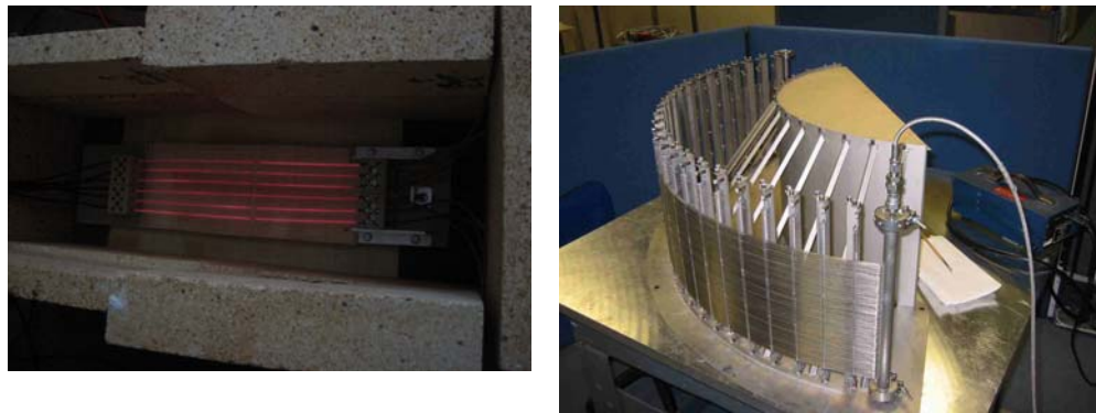
Figure 14 Left: Oxidation testing of Inconel 718 tubes, right: completed precooler module in assembly fixture during pressure testing.
