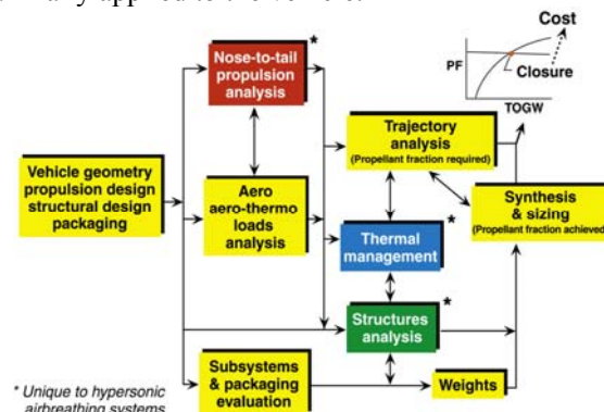
Figure 35: Hypersonic Vehicle Design System [34]
