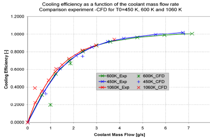
Figure 69: Numerical and experimental cooling efficiency vs. blowing ratio for T_{t,g} = 450 K, 600K and 1060 K.
