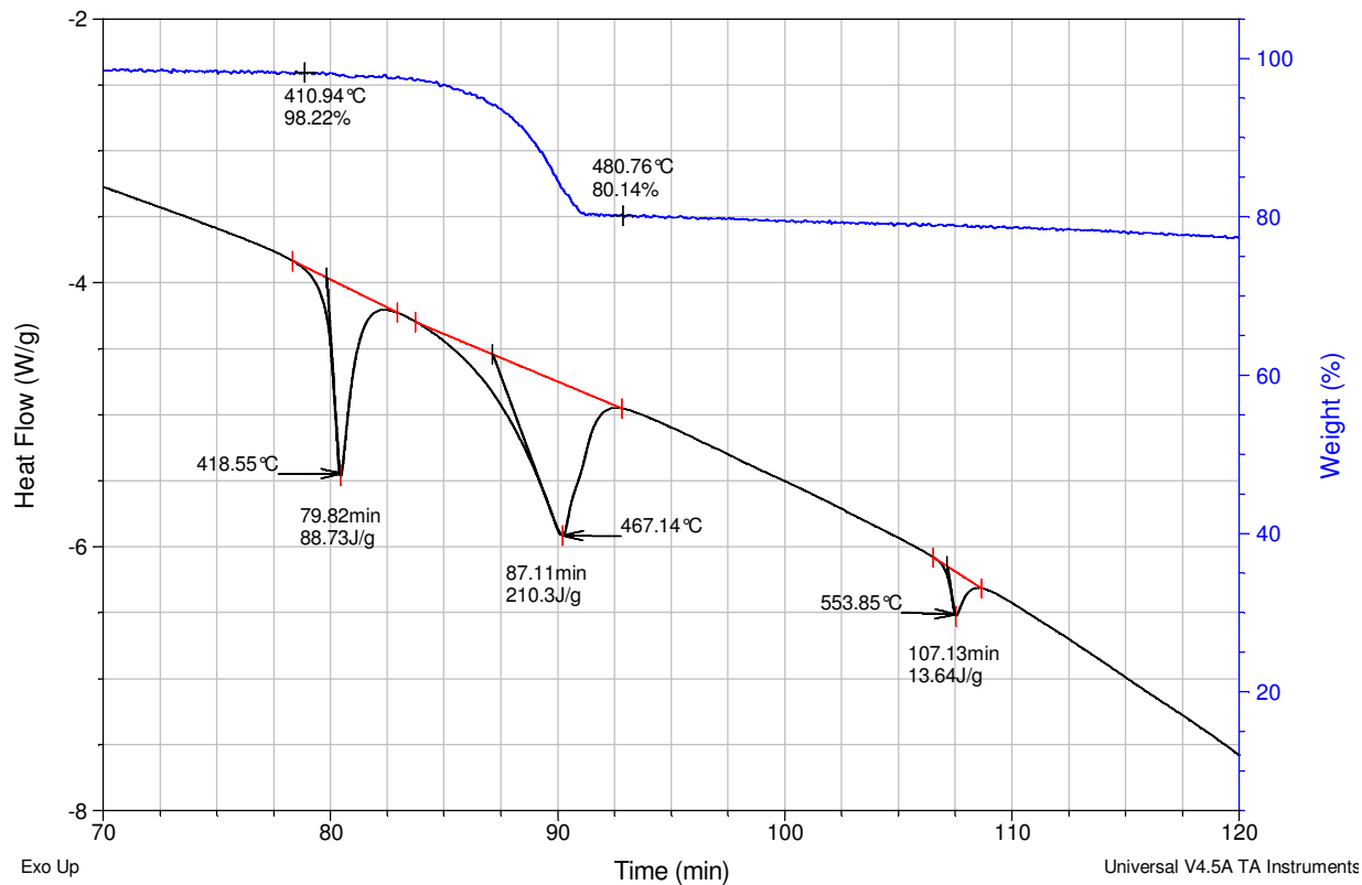
Figure 8.1.1 Thermal analysis by DSC-TGA of AgIO 3 heated under nitrogen at 5 K/min. The AgIO 3 was commercial micron sized AgIO 3 ball milled down to a particle size of around 900 nm. This experiment was run at NAWC China Lake by Curtis Johnson.
