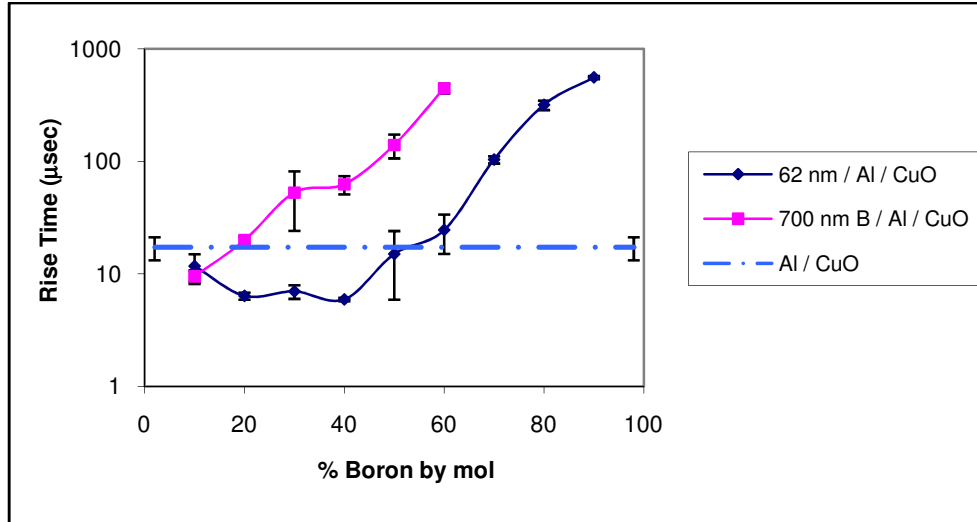
Figure 5.4 Experimental rise times as a function of %B in an Al / B / CuO MIC for both nano and micron-sized boron. The horizontal line is Al / CuO data, included for comparison. Error bars represent the standard deviation of the experimental data.
