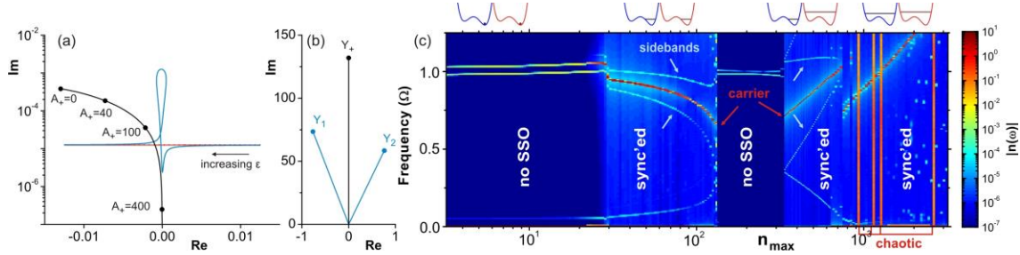
Figure 3. (a) Complex plane representation of the cavity response \Phi(A_+) (black) and the right hand side of Eq. (5) for two identical oscillators (red) and two oscillators with \bar{\gamma} = 0.001 \bar{\Omega} , \bar{c}_{om} = 20 , \nu = 0.01 \bar{\Omega} , \delta\gamma = 0.0018 \bar{\Omega} , and \delta c_{om} = 0 (blue). The curves intersect at A_+ = 132.0 and \epsilon = 0.0438 \bar{\Omega} (b) Complex amplitudes of the individual oscillators for the solution shown in (a). (c) Colorplot of the Fourier transform of the photon number on a logarithmic scale. The carrier tone and its sidebands are indicated by red and white arrows respectively. The parameters are: Q_1 = Q_2 = 6000 , \kappa = 526 \bar{\Omega} , \Delta_0 = 0.493\kappa , g_{om,1} = g_{om,2} = 1 .
