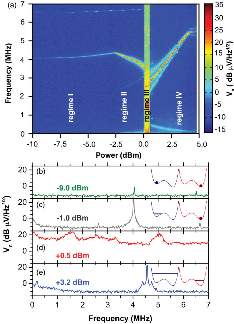
Figure 2. (a) The evolution of the RF power spectrum of the transmitted light as the pump power increases. (b)-(e) Cuts through panel (a) at the indicated pump power when both resonators are in a thermal state (regime I, (b)), (c) one resonator is in thermal motion while the other resonator experiences regenerative oscillations (regime II), (d) the chaotic regime (III) and (e) the two resonators are synchronized (regime IV). The insets schematically show the energy of resonators 1 (left) and 2 (right); dots correspond to small thermal motion, and lines to large oscillations.
