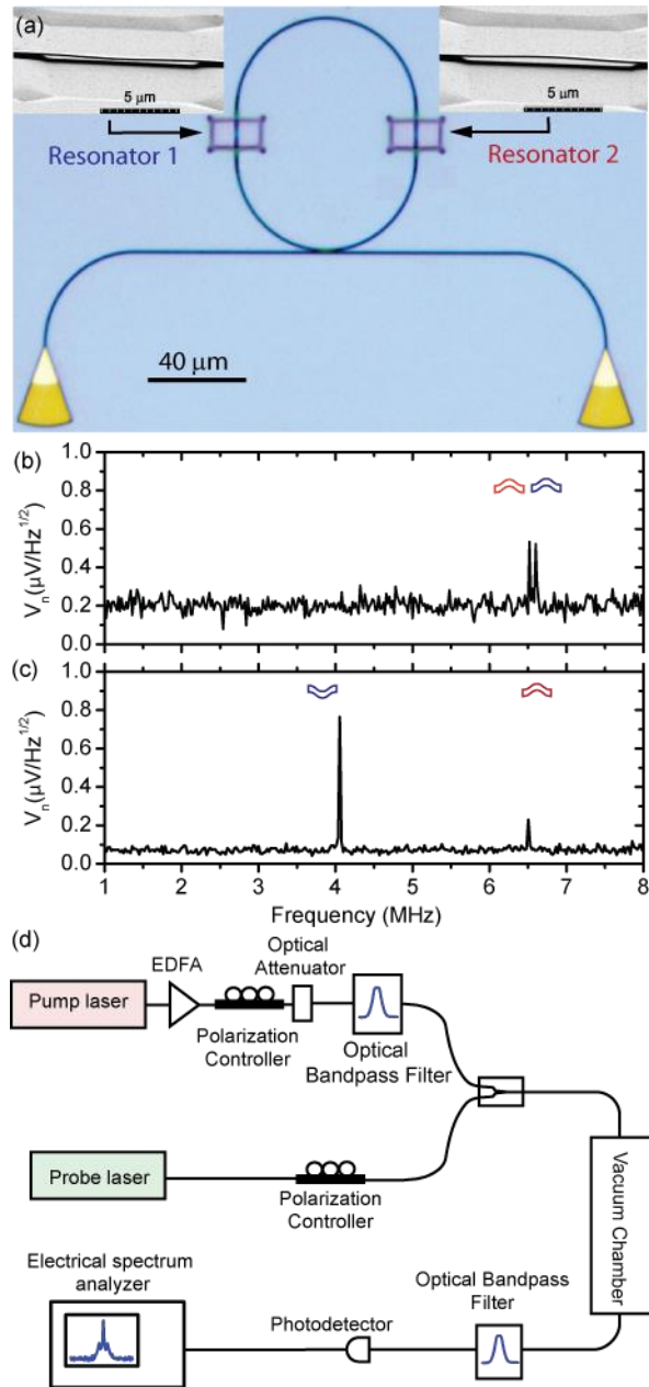
Figure 1. (a) Micrograph of a racetrack cavity with two 110nm x 500nm x 10μm suspended portions as nanomechanical resonators. Insets show scanning electron micrographs of the mechanical resonators in buckled down (left) and buckled up (right) state. (b,c) thermal noise spectra in the up-up (b) down-up state (c). (d) The measurement setup with a weak probe laser, and a pump.
