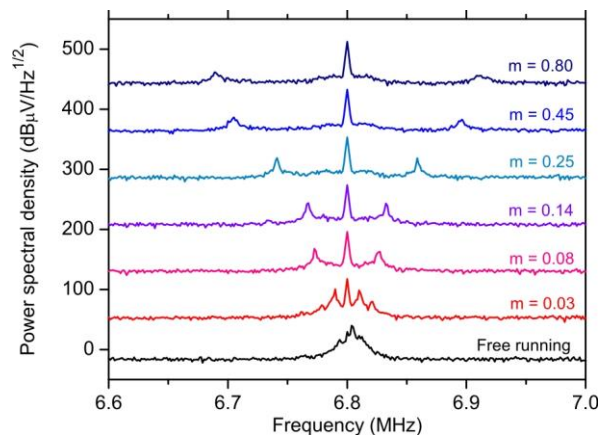
Figure 4. Measured RF power spectral density of the detector output with a free running oscillator (black) and oscillations in the presence of an increasingly larger modulation depth of the pump (red to dark blue) for constant average power. The curves are offset for clarity.
