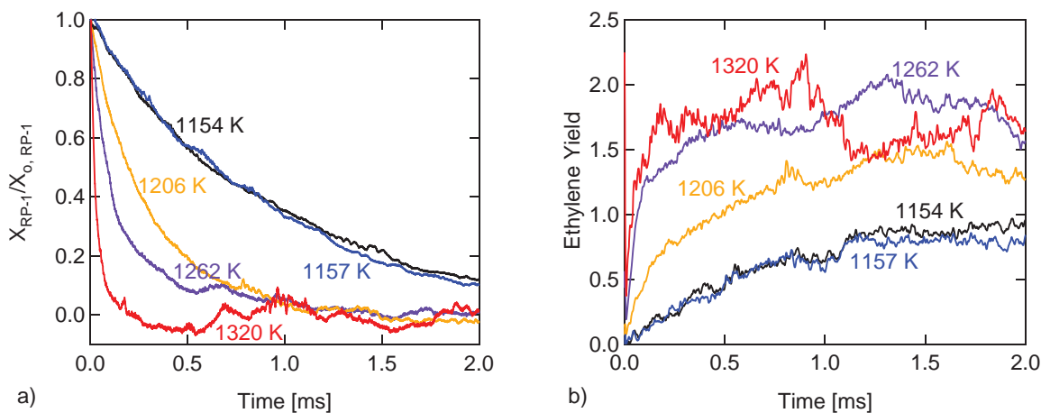
Fig. 5 RP-1 decomposition. Initial reflected shock conditions: 1051 - 1320 K, 18.4 - 20.4 atm, 0.14 - 0.17% fuel in argon. a) Normalized RP-1 mole fraction. b) Ethylene yields. Uncertainty (as shown Fig. 4) is \pm 100 ppm for RP-1 and \pm 500 ppm for ethylene.
