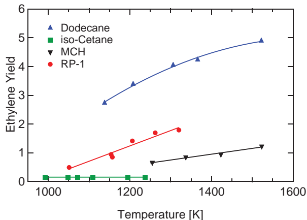
Fig. 7 Ethylene yields during decomposition of RP-1 and three possible surrogate components. Solid lines are best fits to the data. Dodecane, iso-Cetane, and MCH data from [MacDonald 2012].
