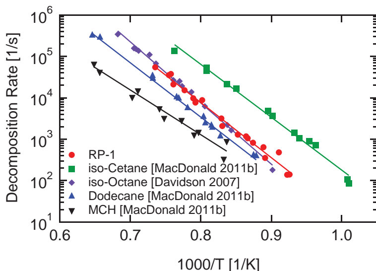
Fig. 6 Decomposition rates of RP-1 and possible surrogate components
