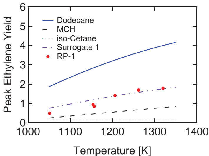
Fig. 10 Comparison of measured RP-1 ethylene yields with the linear combination of the measured overall ethylene yields from the surrogate components. Dodecane, iso-Cetane, and MCH data from [MacDonald 2012].
