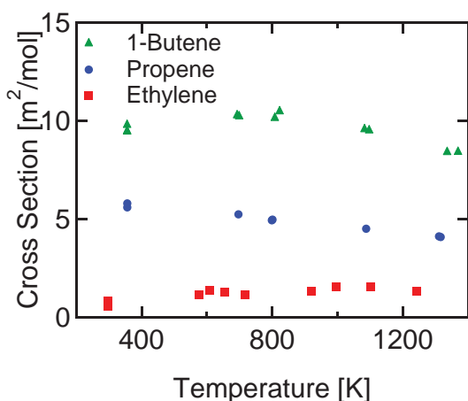
Fig. 1 Absorption cross sections of small alkenes at 3.39 \mu\text{m} (20 atm).
