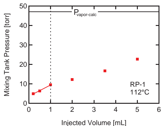
Fig. 3 HPST mixing tank complete evaporation check. Tank temperature 112°C, tank volume 12.84 L. Solid curve is a fit to the data. The beginning of the roll-off is indicated by the dashed line, and occurs at about 1 mL.
