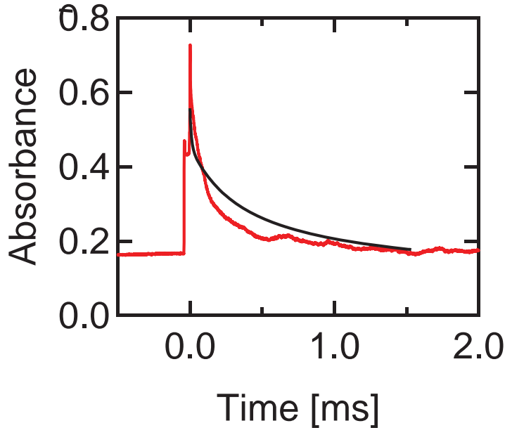
Fig. 11 Measured and predicted absorbance for initial reflected shock conditions: 3.39 \mu\text{m} , 1262 K, 18.4 atm, 0.17% RP-1 in argon.
