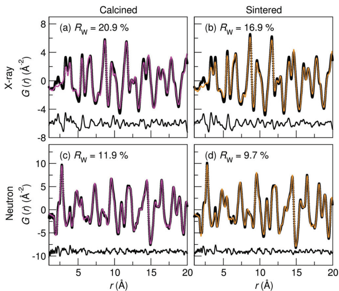
FIG. 3. (Color online) Results of fitting 1–20 Å x-ray G(r) s (a),(b) and neutron G(r) s (c),(d) with the Cc average structure model for sintered and calcined NBT samples. Data are shown as black circles, fits are given as purple and orange lines (for calcined and sintered samples, respectively), and difference curves have been offset below the data and fits in black. Refined goodness of fit parameters ( R_w ) are given in each panel. Note x-ray and neutron data are shown on different intensity scales.
