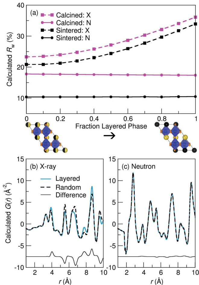
FIG. 4. (Color online) Exploring A -site ordering: (a) 10 \text{\AA} PDF refinement R_w values (goodness of fit) for sintered (black) and calcined (purple) data sets with different fractions of mixed-site A -cation and layered A -cation structure models. Neutron results are given with circles and solid lines through the points, while x-ray results are given with squares and dashed lines through the points. In the bottom two panels, 10 \text{\AA} x-ray (b) and neutron (c) PDF calculations are displayed for the two end-member model structures (at fraction of layered phase = 0 and 1). The random structure calculations are shown in black dashed lines and the layered structure calculations are displayed in blue solid lines.
