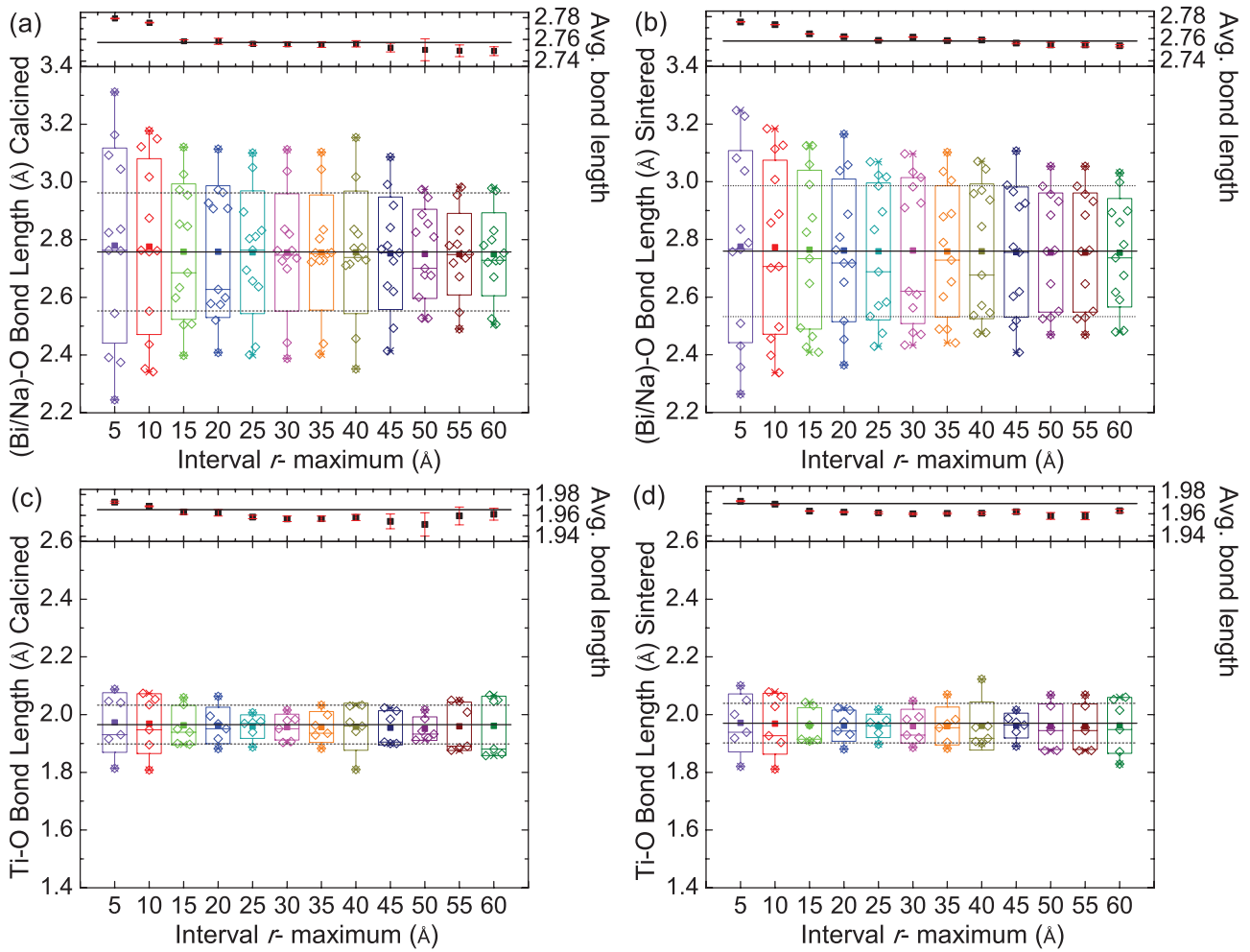
FIG. 5. (Color online) Calculated (Bi/Na)-O (a) and (b) as well as Ti-O (c) and (d) bond lengths from the box-car fitting method are shown for both calcined and sintered NBT. The box plots at each r value indicate the spread in the bond lengths for that calculation. The edges of the box represent one standard deviation from the mean and the whiskers are the minimum and maximum values. The closed symbols for each data set are the mean values while the open symbols show all of the bond lengths. The solid line in each plot is the average bond length calculated from the atomic positions refined through the Rietveld method and the dashed lines show one standard deviation from the mean. The inset in each plot shows the average bond lengths from the box-car fitting on a smaller y scale for clarity (all insets have the same y range).
