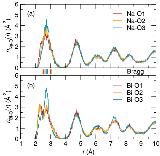
FIG. 9. (Color online) Partial pair distribution functions from the RMC model of a sintered sample give nearly symmetric bond distance distributions of Na-O (a). Tick marks between the two panes show the Rietveld-refined bond distances in the Cc cell. For Bi-O in (b), the asymmetry seen in the Cc cell is greatly amplified. Distances are shown to each of the three distinct O atoms on 4a sites in the Cc cell. Results for calcined samples were similar.
