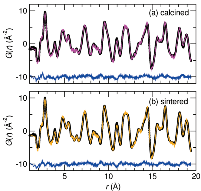
FIG. 7. (Color online) Reverse Monte Carlo fits to the neutron PDF of (a) calcined and (b) sintered NBT. Data are shown as black dots, fits as colored lines, and a difference curve falls below. Both simulations are conducted with BVS constraints to maintain the nominal cation valences.
