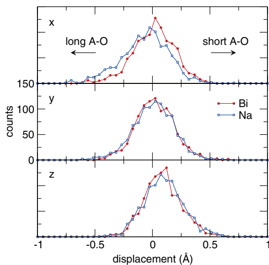
FIG. 10. (Color online) The distribution of the \text{Na}^+ and \text{Bi}^{3+} ions relative to the average A -site position. The x and y directions are along the a and b unit cell axes, and z is orthogonal to them.
