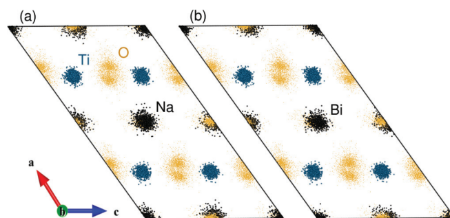
FIG. 8. (Color online) Folded RMC models produce “point clouds” of atoms at each crystallographic site. No significant differences are seen when a single model is plotted to show only \text{Na}^+ (a) and \text{Bi}^{3+} (b) cations, implying that \text{Bi}^{3+} does not simply displace off-center, and does not have significantly larger displacement than \text{Na}^+ .
