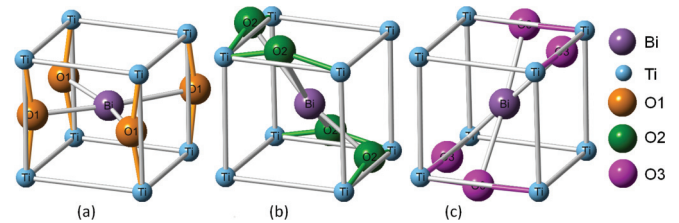
FIG. 11. (Color online) Pseudocubic representation of the NBT unit cell showcasing the arrangement of the three unique oxygen lattice positions relative to the Bi site: (a) O1, (b) O2, and (c) O3 positions.
