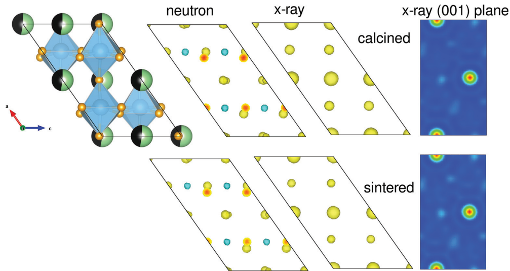
FIG. 2. (Color online) The NBT unit cell is shown on the left, where the green and black circles represent the A site, the O sites are shown as orange circles, and the Ti site is in the center of the blue octahedron. The four figures in the middle are Fourier maps represented as three-dimensional isosurfaces showing the total scattering density in the NBT unit cell for neutron and x-ray Bragg profiles. Only the A site and Ti site are shown for x-ray maps, while the neutron maps include O sites. The light blue surfaces in the neutron maps indicate the negative scattering density of Ti. X-ray scattering densities on the A sites are shown on the far right along the monoclinic (001) plane, with only spherical intensity present.
