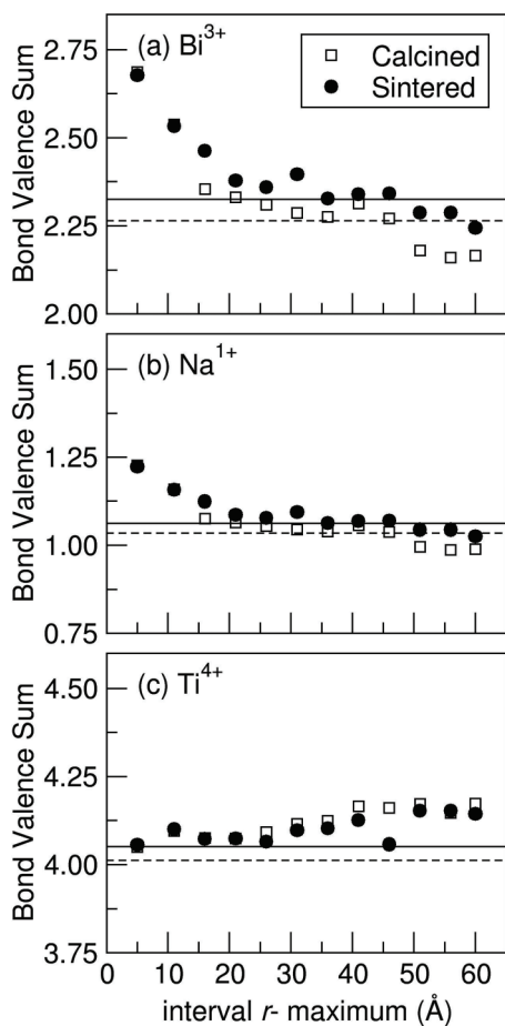
FIG. 6. The calculated BVS for \text{Bi}^{3+} (a), \text{Na}^+ (b), and \text{Ti}^{4+} (c) is shown for the calcined and sintered materials. The dashed and solid lines in the plots represent the BVS calculated from the average structure obtained by the Rietveld method for calcined and sintered NBT, respectively. The y axis scales are identical in all three panels.
