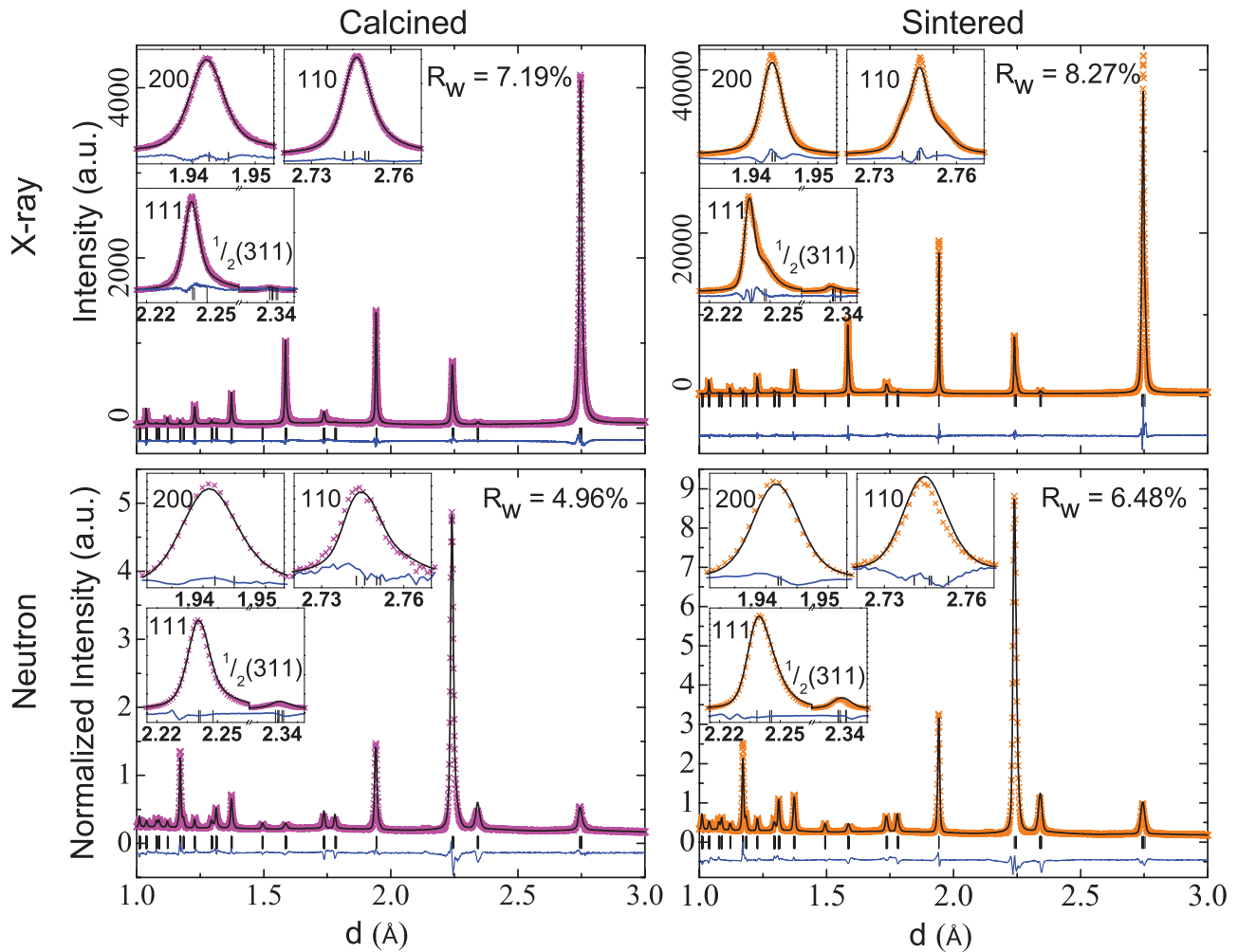
FIG. 1. (Color online) Powder diffraction patterns of sintered (orange \times ) and calcined (pink \times ) NBT powders from neutron and x-ray diffraction. The results of a calculated fit (—) using both the x-ray and neutron diffraction patterns for each type of powder are also shown. Reflection markers for the Cc phase are shown as vertical lines with the difference pattern below the diffraction pattern. The labeled peak indices are relative to the pseudocubic perovskite unit cell. The refined Bragg R values ( R_w ) of each fit are also indicated in the figure.
