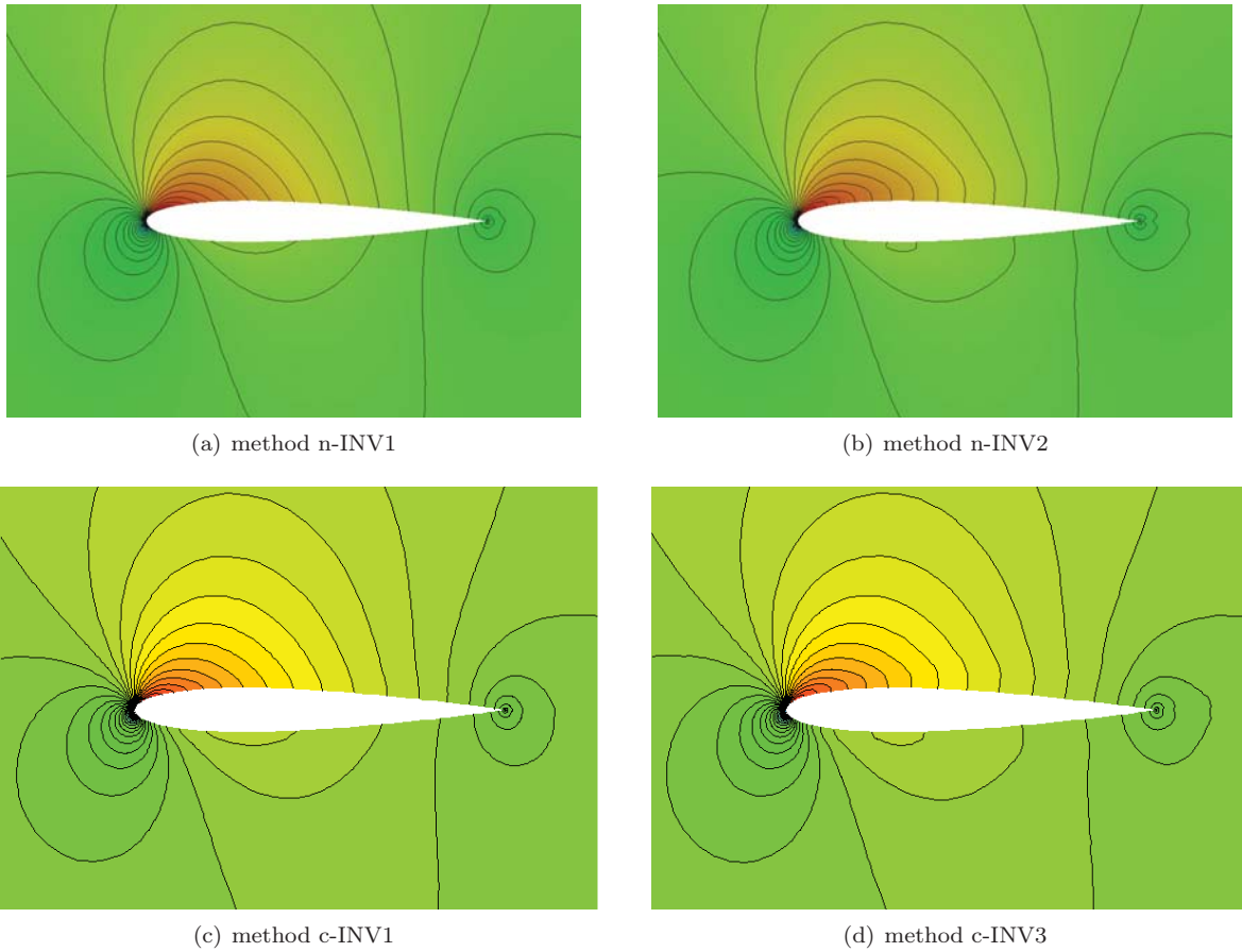
Figure 11: Mach contours for various inviscid wall treatments of a NACA 0012 inviscid airfoil at M = 0.5 , \alpha = 3.0^\circ .
