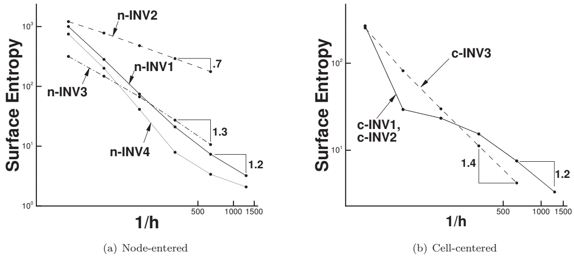
Figure 10: Grid refinement study for various boundary formulations using flow around a NACA 0012 airfoil.
