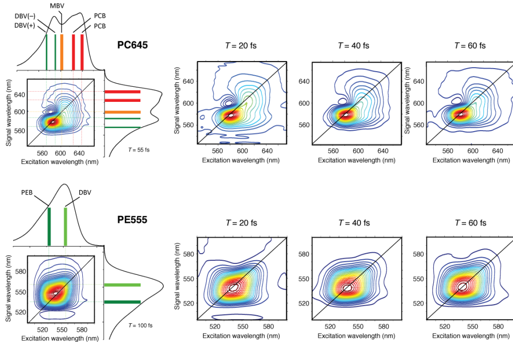
Figure 1. Representative 2D spectra of PC645 and PE555 plotted at various waiting times ( T ) with corresponding linear absorption spectra shown alongside the T = 55 fs spectrum of PC645 and the T = 100 fs spectrum of PE555. The 2D spectra are the real part of the total signal, plotted with 33 evenly-spaced contours. The colored bars in the linear spectra indicate locations of the estimated peak transition energies of individual components.
