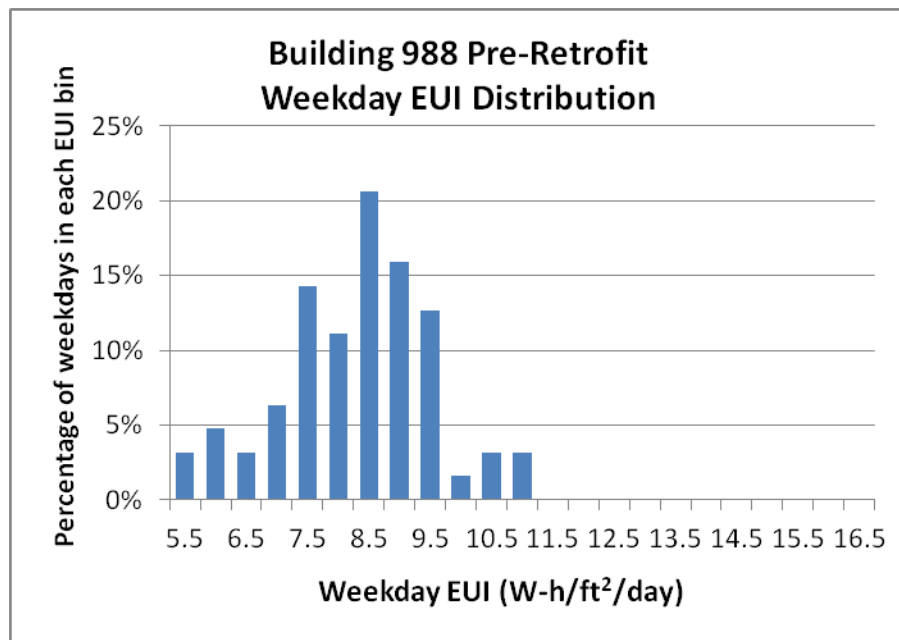
Figure 39: Pre-retrofit weekday EUI in building 988
