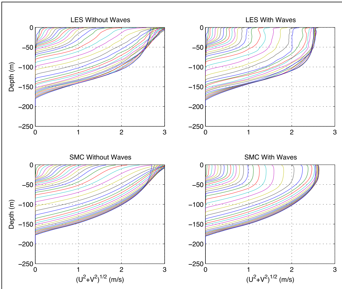
Fig. 2. Simulations of upper ocean shear below the passage of a tropical cyclone, compared between the new second moment closure (SMC) and turbulence-resolving LES, both with and without including the Craik-Leibovich effect due to the Stokes drift of surface waves.
