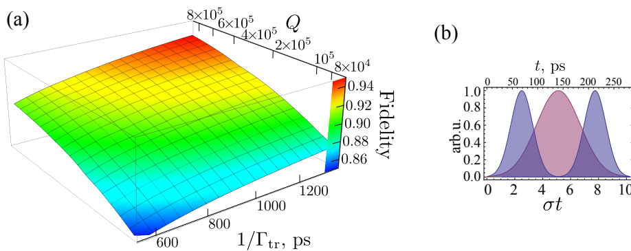
FIG. 3: (a) Fidelity of the two-qubit CZ gate in presence of decoherence due to trion recombination and cavity decay. The fidelity is plotted as a function of the trion decay time and the cavity mode quality factor. (b) The temporal profiles of the pulse sequence for \sigma/\omega_e = 0.2 , \omega_h = \omega_e/3 , \Delta\varepsilon/\omega_e = 8.33 , g/\omega_e = 3.33 , and \omega_e = 0.12\text{meV} .
