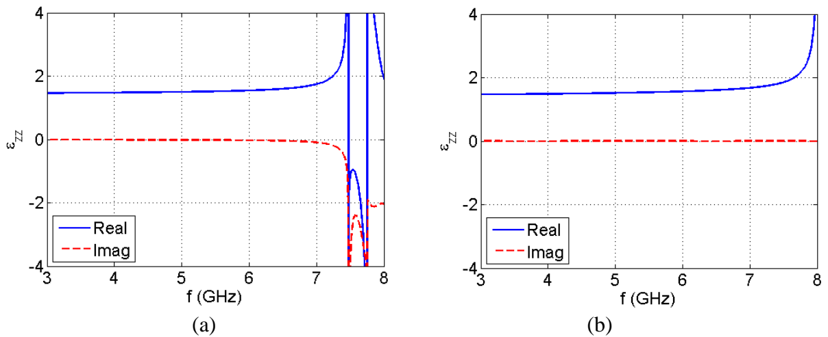
Figure 4.9. Extracted \epsilon_{zz} for the structure in Fig. 4.6; (a) TE2 way, (b) TM3 way of retrieval of effective parameters (definitions are given in Fig. 3.10 and Table 3.3).
