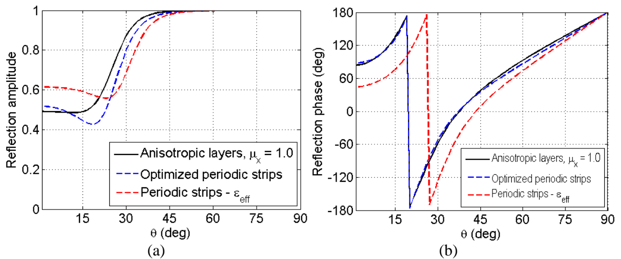
Figure 4.2. Amplitude and phase of reflection coefficient of an anisotropic dielectric multilayer structure and of metamaterial realization. Anisotropic layer is characterized with constitutive parameters given in Table 4.1 (permeability \mu_x = 1.0 ). The width of the strips is given in Table 4.2.
