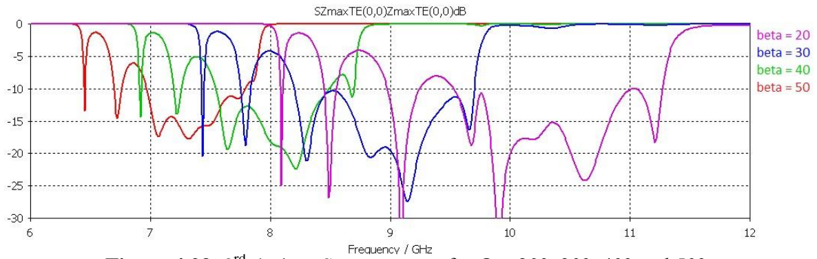
Figure 4.29. 3 rd design: S_{11} parameter for \beta = 20^\circ, 30^\circ, 40^\circ and 50^\circ
