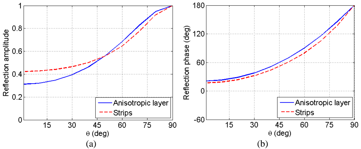
Figure 3.18. Amplitude and phase of reflection coefficient of an anisotropic dielectric layer and of metamaterial realization. Anisotropic layer is characterized with \epsilon_x = \epsilon_z = 1.0 , \epsilon_y = 0.5 and with \mu_x = 1.0 . The used cost function in optimization routine is defined by eq. (3.25). Parameters of strips are listed in Table 3.4.
