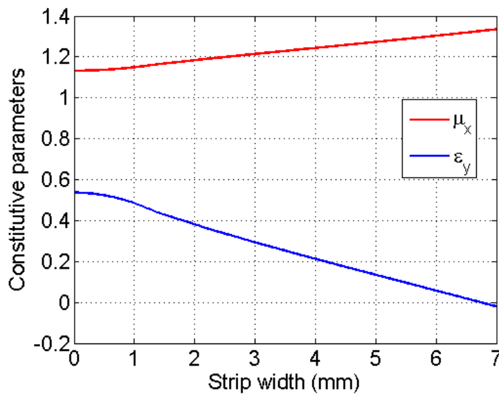
Figure 3.15. Effective constitutive parameters of a dielectric slab with periodic metal strips
