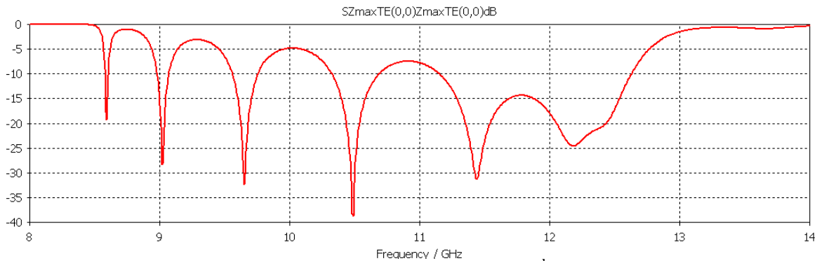
Figure 4.16. S_{11} parameter of the 2 nd design
