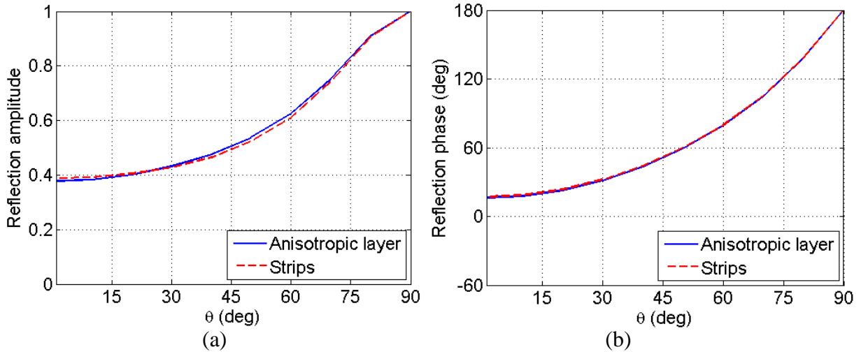
Figure 3.21. Amplitude and phase of reflection coefficient of an anisotropic dielectric layer and of metamaterial realization. Anisotropic layer is characterized with \epsilon_x = \epsilon_z = 1.0 , \epsilon_y = 0.5 and with \mu_x = 1.146 . The used cost function in optimization routine is defined by eq. (3.26). Parameters of strips are listed in Table 3.4.
