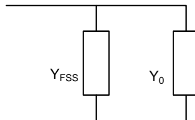
Figure 3.11. Equivalent network of FSS in free-space.
