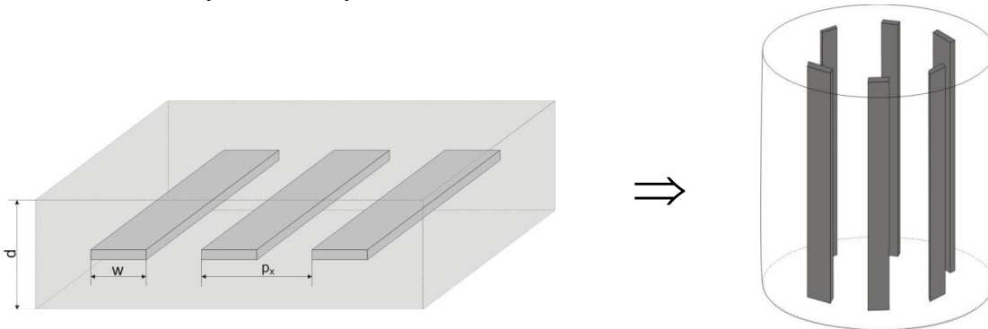
Figure 3.23. Transformation of planar to cylindrical metamaterial structure.
