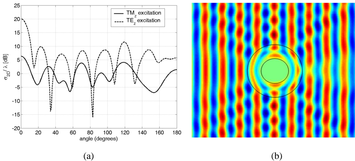
Figure 3.8. (a) Normalized bistatic scattering width ( TM_z and TE_z polarizations) and (b) electric field distribution in the vicinity of the cloaked object ( TM_z polarization) of 10-layers realization of TM_z cloak.
