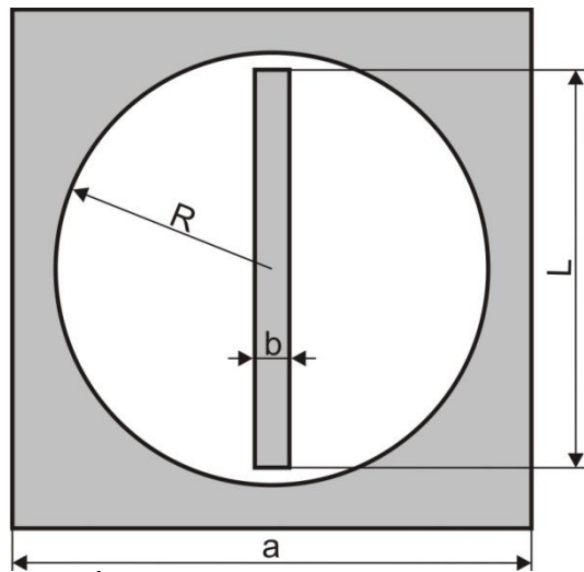
Figure 4.15. 2 nd design: dipole in a slot surrounded by metal ( a=10 mm, L=8 mm, R=4.5 mm, b=1 mm)
