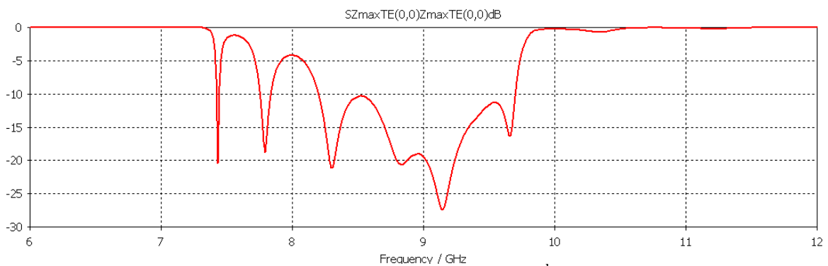
Figure 4.24. S_{11} parameter of the 3 rd design
