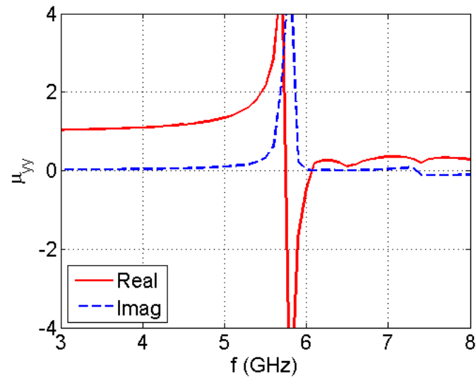
Figure 4.10. Extracted \mu_{yy} of the structure in Fig. 4.6 obtained by the Moment Method.
