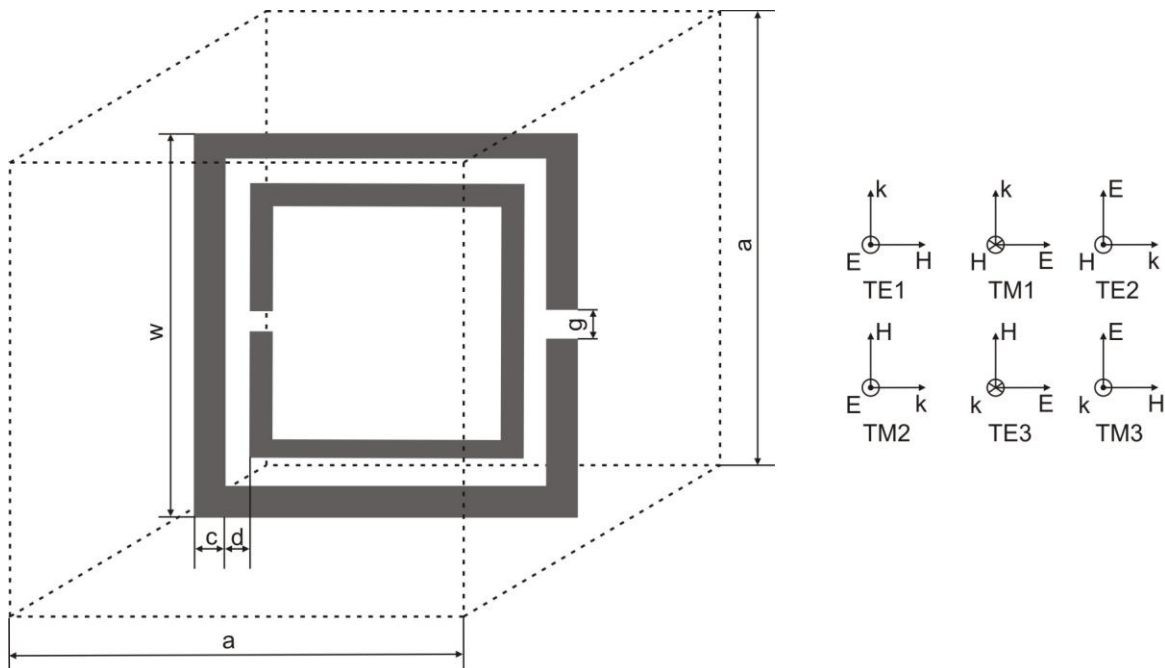
Figure 3.10. S-matrix approach for determining constitutive parameters. The method is based on measuring or calculating S_{11} and S_{21} for six test cases.
