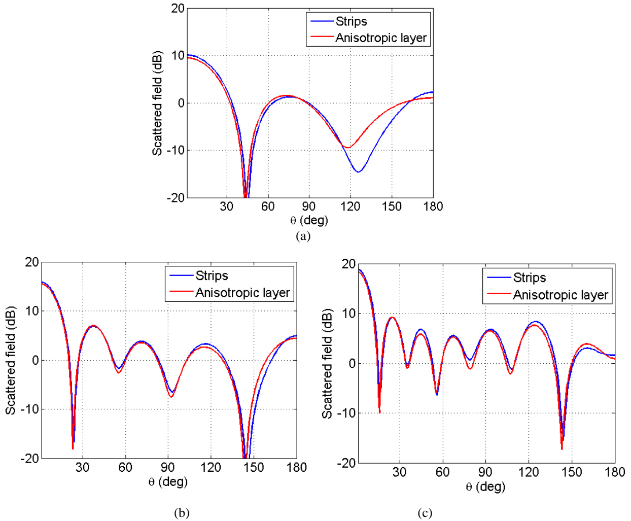
Figure 3.24. Scattered field from the periodic strip-grid structure and from the homogeneous anisotropic cylindrical shell. (a) \rho_{strips} \cong 0.5 \lambda_0 , (b) \rho_{strips} \cong 1.0 \lambda_0 , (c) \rho_{strips} \cong 1.5 \lambda_0 .
