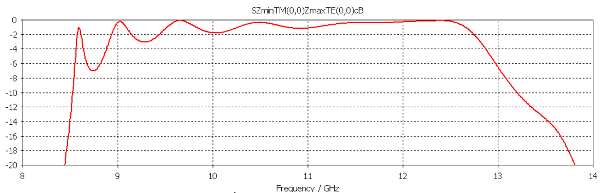
Figure 4.18. S_{21} parameter of the 2 nd design, coupling between TE input and TM output wave
