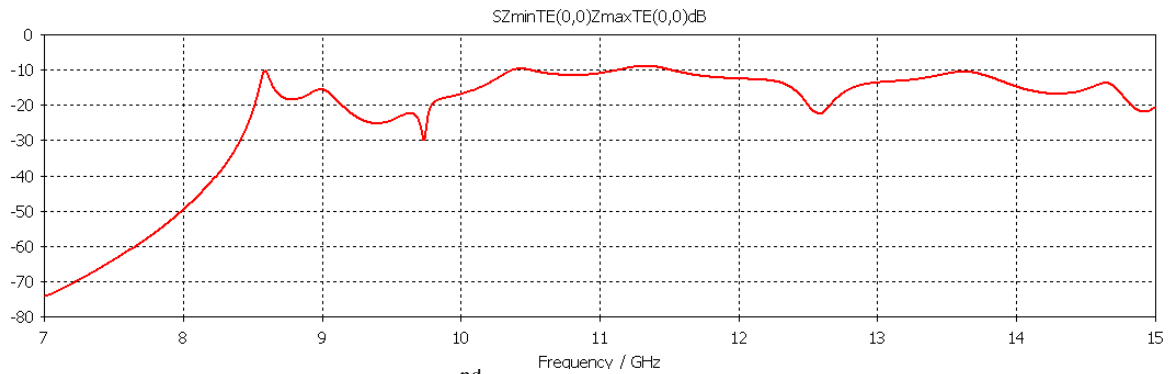
Figure 4.17. S_{21} parameter of the 2 nd design, coupling between TE input and output waves
