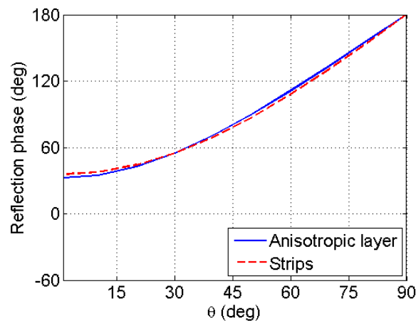
Figure 3.16. Phase of reflection coefficient of a grounded anisotropic dielectric layer and of metamaterial realization. Anisotropic layer is characterized with \epsilon_x = \epsilon_z = 1.0 , \epsilon_y = 0.5 and \mu_x = 1.0 . The used cost function in optimization routine is defined by eq. (3.24). Parameters of strips are listed in Table 3.4.
