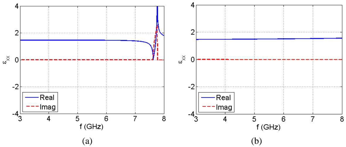
Figure 4.8. Extracted \epsilon_{xx} for the structure in Fig. 4.6; (a) TM1 way, (b) TE3 way of retrieval of effective parameters (definitions are given in Fig. 3.10 and Table 3.3).
