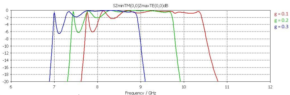
Figure 4.28. 3 rd design: S_{21} parameter for g=0.1 mm, 0.2 mm and 0.3 mm; coupling between TE input and TM output wave is considered.
