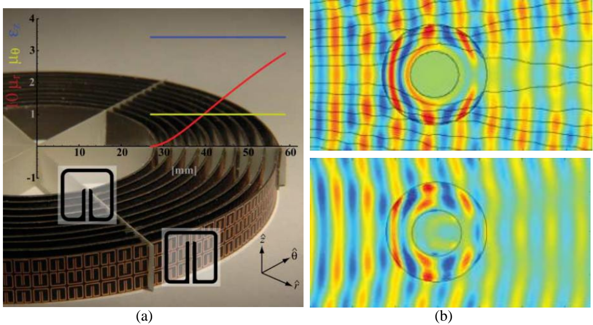
Figure 3.3. (a) sketch of the first experimentally developed cloak, (b) calculated and measured scattered field (Schurig et al. , 2006 [16]).
