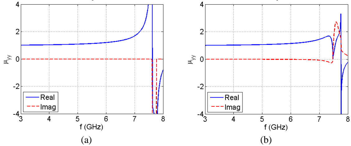
Figure 4.7. Extracted \mu_{yy} for the structure in Fig. 4.6; (a) TE2 way, (b) TM1 way of retrieval of effective parameters (definitions are given in Fig. 3.10 and Table 3.3).
