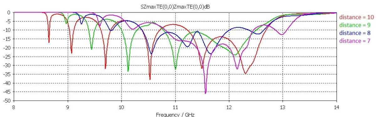
Figure 4.19. S_{11} parameter as a function of distance between neighboring screens (distance is 10mm, 9 mm, 8 mm and 7 mm, respectively)
