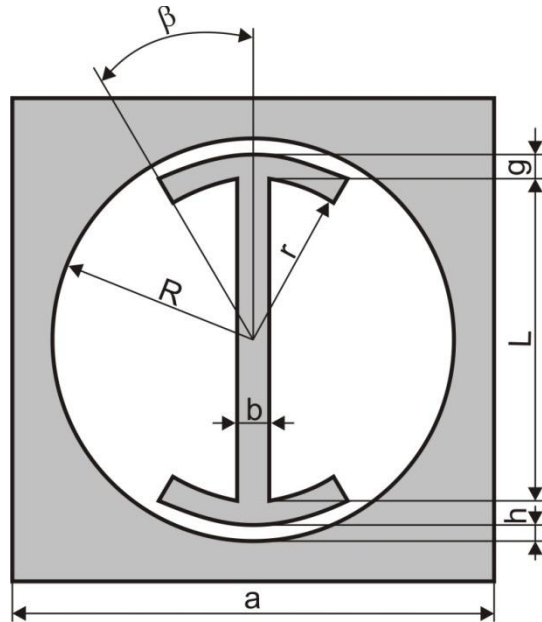
Figure 4.23. 3 rd design: dipole in the slot surrounded with metal. An arch at the top and bottom of dipole are introduced to increase capacitance ( g=0.2, \beta=45 )
