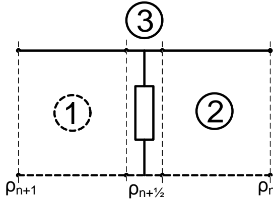
Figure 3.25. Decomposition of periodic unit cell into 3 parts.
