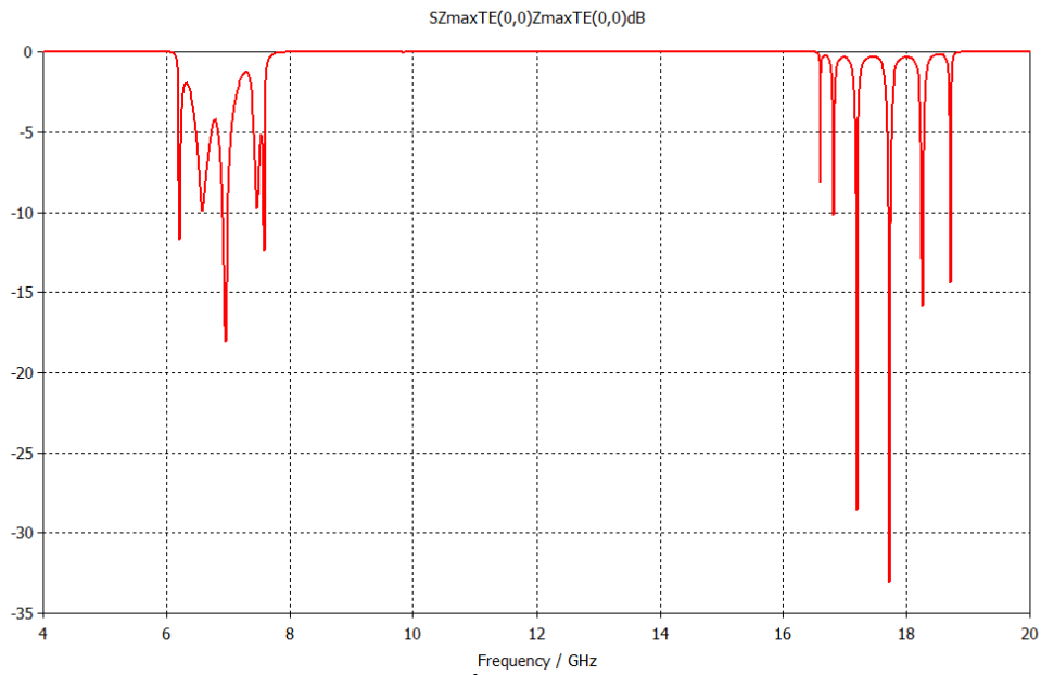
Figure 4.32. 4 th design: S_{11} parameter
