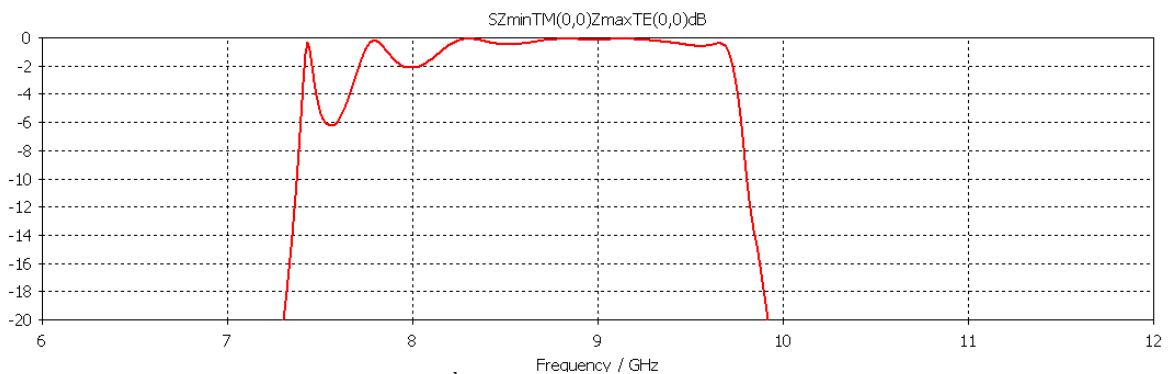
Figure 4.25. S_{21} parameter of the 2 nd design, coupling between TE input and TM output wave
