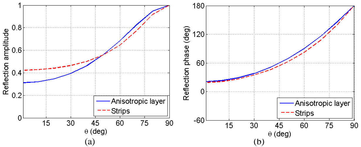
Figure 3.20. Amplitude and phase of reflection coefficient of an anisotropic dielectric layer and of metamaterial realization. Anisotropic layer is characterized with \epsilon_x = \epsilon_z = 1.0 , \epsilon_y = 0.5 and with \mu_x = 1.0 . The used cost function in optimization routine is defined by eq. (3.26). Parameters of strips are listed in Table 3.4.
