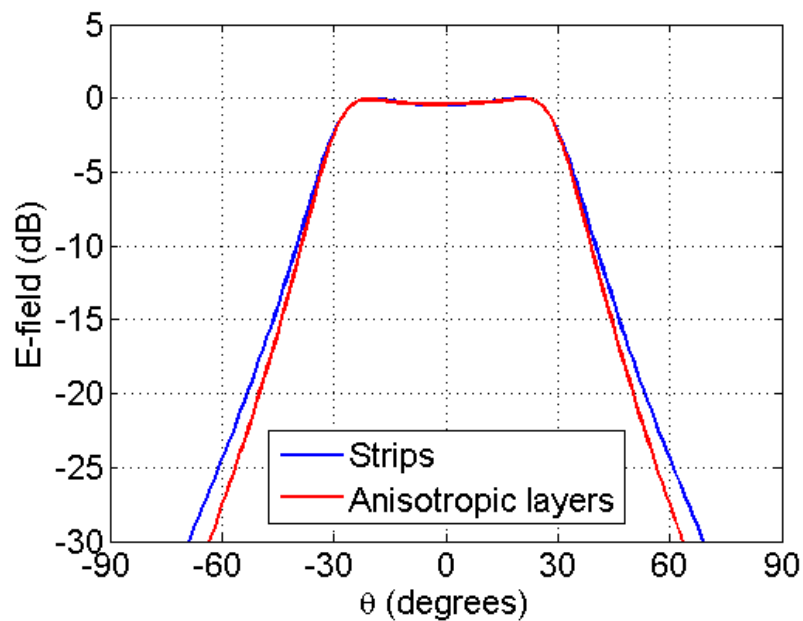
Figure 4.5. H-plane radiation pattern of a dipole antenna with planar metamaterial lens.
