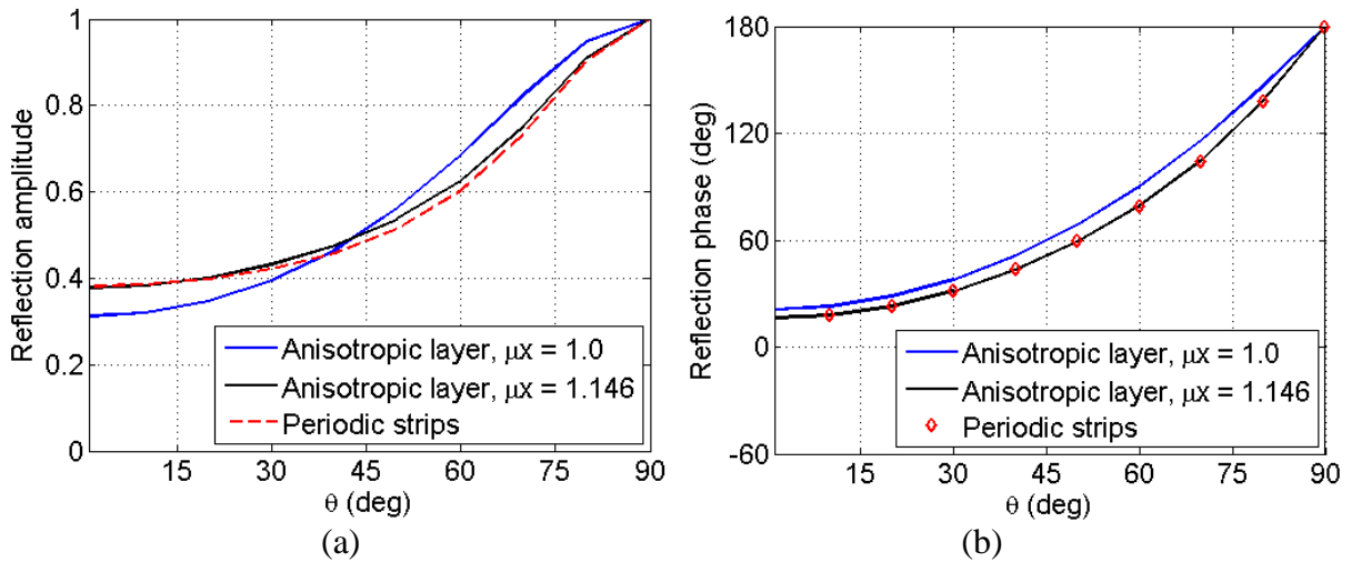
Figure 3.22. Amplitude and phase of reflection coefficient of an anisotropic dielectric layer and of metamaterial realization. Anisotropic layer is characterized with \epsilon_x = \epsilon_z = 1.0 , \epsilon_y = 0.5 and with \mu_x = 1.146 . The width of the strips is determined using effective constitutive parameters approach.
