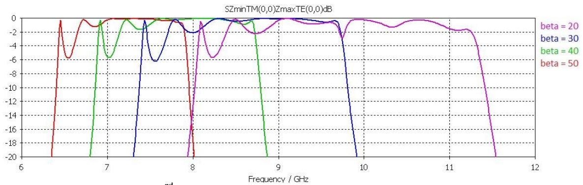
Figure 4.30. 3 rd design: S_{21} parameter for \beta = 20^\circ, 30^\circ, 40^\circ and 50^\circ ; coupling between TE input and TM output wave is considered.
