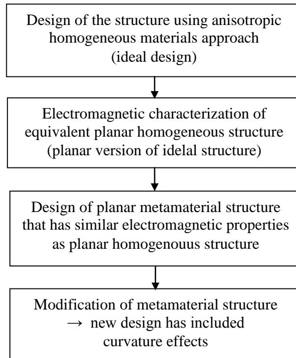
Figure 3.12. The proposed designing procedure of metamaterial structures
