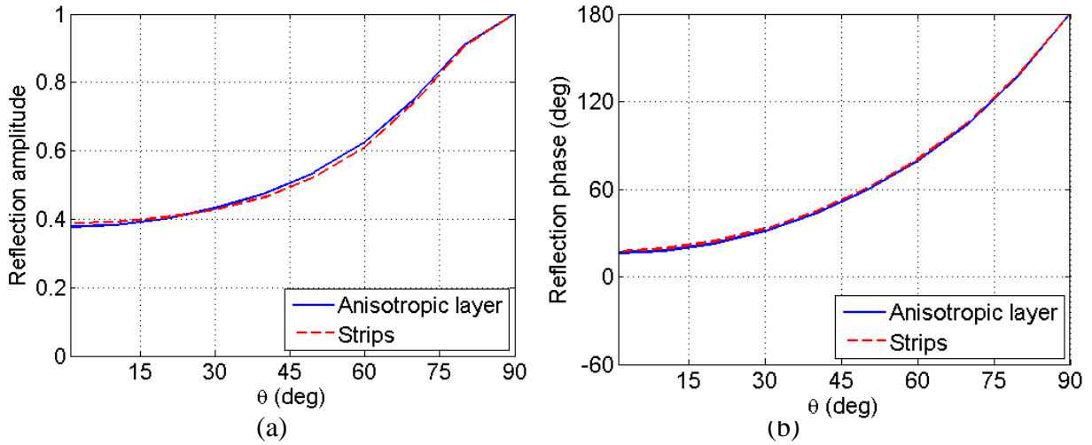
Figure 3.19. Amplitude and phase of reflection coefficient of an anisotropic dielectric layer and of metamaterial realization. Anisotropic layer is characterized with \epsilon_x = \epsilon_z = 1.0 , \epsilon_y = 0.5 and with \mu_x = 1.146 . The used cost function in optimization routine is defined by eq. (3.25). Parameters of strips are listed in Table 3.4.
