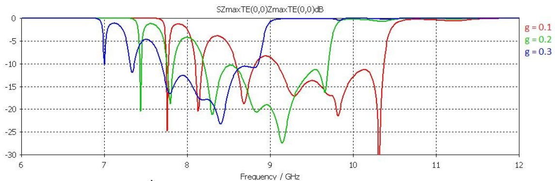
Figure 4.27. 3 rd design: S_{11} parameter for g=0.1 mm, 0.2 mm and 0.3 mm.
