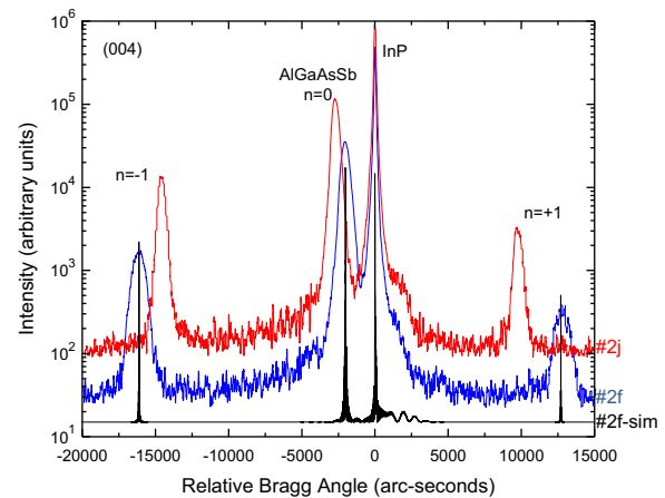
Fig. 4. X-ray diffraction data for samples #2f and 2j and simulation for 2f. The lattice parameter of the buffer layer (and the strain in the channel and barrier layers) is extracted from the peak separations.
