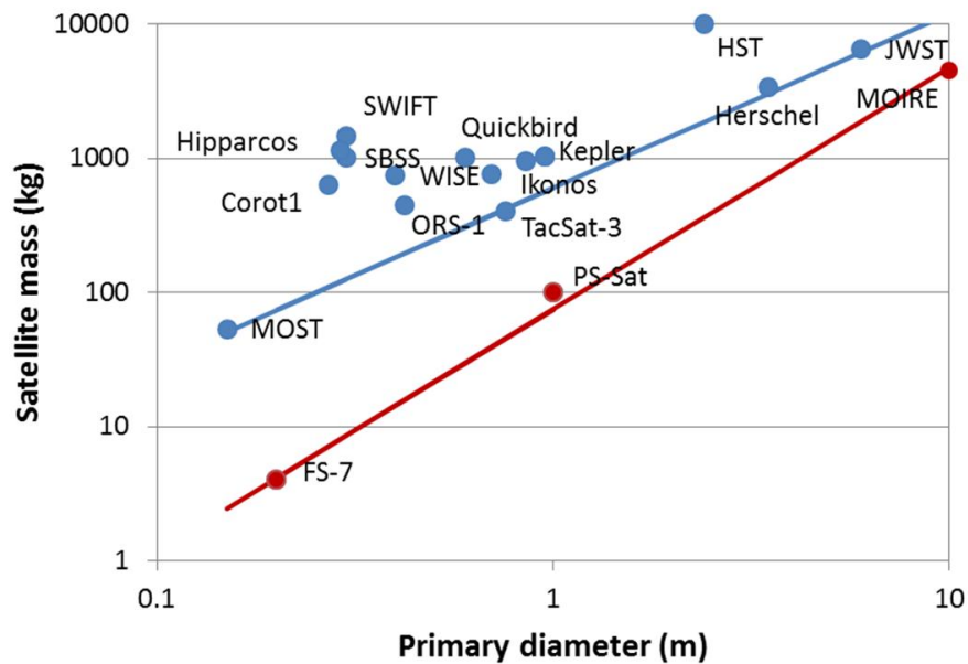
Fig. 1. A plot of current space telescopes (blue) compared to planned satellites using diffractive membrane primaries (red).
