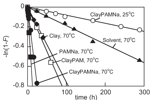
Figure 7. Typical kinetics of parathion hydrolysis at pH 8.6 and T = 25 or 70\text{ }^\circ\text{C} . Solvent: 50 mM CHES/ \text{D}_2\text{O} buffer (27 wt %) in acetonitrile. Initial concentration of parathion, 6.5 mM. Hydrolytic species designations: Clay (montmorillonite K-10), ClayPAM (montmorillonite K-10 functionalized with pralidoxime methiodide, pH 3.2), ClayPAMNa (montmorillonite K-10 functionalized with pralidoxime methiodide, pH 8.6), PAMNa (pralidoxime methiodide obtained by drying pralidoxime methiodide solution with pH adjusted to 8.6 by sodium methoxide).
