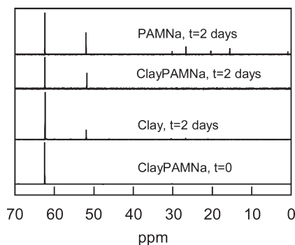
Figure 6. Typical ^{31}\text{P} NMR spectra of parathion degradation at pH 8.6, 70\text{ }^\circ\text{C} and time points taken at t = 0 or 2 days. Solvent: 50 mM CHES/ \text{D}_2\text{O} buffer (27 wt %, pH 8.6) in acetonitrile. Initial concentration of parathion, 6.5 mM. Hydrolytic species are added at 4 mg/mL concentrations. Designations: Clay (montmorillonite K-10), ClayPAMNa (montmorillonite K-10 functionalized by sodium pralidoxime, pH 8.6), PAMNa (pralidoxime methiodide obtained by freeze-drying PAM solution with pH adjusted to 8.6 by sodium methoxide). At t = 0 , identical spectra without the hydrolysis products were observed in the presence or absence of functionalized clays or PAMNa (not shown for clarity).
