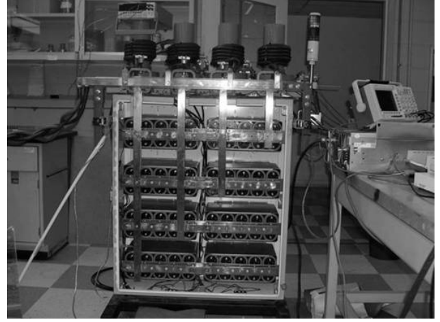
Fig 2. 28 kJ Pulsed power supply.
