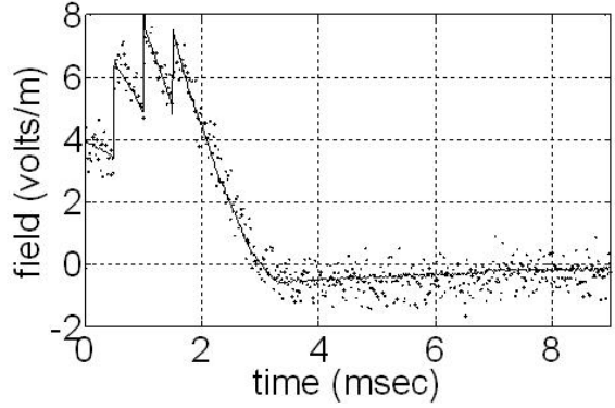
Fig. 6. Theoretical (solid line) and measured (points) rail-to-rail field values using 0.5 ms staging. R_X = 75 \mu\Omega/\text{m} L_X = 0.56 \mu\text{H/m} , and r^2 = 0.97 .
