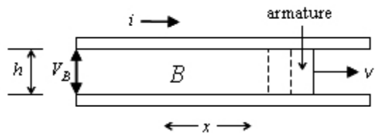
Fig.1. Schematic of a simple railgun.
