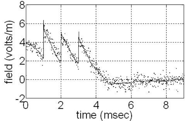
Fig. 7. Theoretical (solid line) and measured (points) rail-to-rail field values using 1.0 ms staging. R_X = 73 \mu\Omega/\text{m} L_X = 0.56 \mu\text{H/m} , and r^2 = 0.95 .
