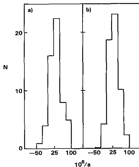
FIG. 1. (a) The observed distribution of 10^6/a for those comets clearly classified as "new"; (b) the simulated distribution in the same parameter from the model in the text. The values of 1/a_{orig} were taken from Marsden et al. (1978).
