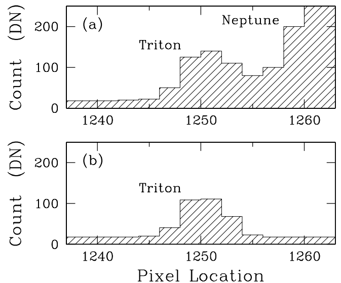
FIG. 8.—Most image centering algorithms assume a flat sky background. When observing satellites near a bright planet (many satellites of planets from Jupiter to Neptune fall into this category), the glare of the planet will cause a steep gradient in the sky level that can, in turn, adversely bias the centroid for a satellite. In the FASTT program, images are corrected for variable background levels, before a two-dimensional Gaussian fit is used to determine their image centers. (a) Cross-sectional view of a FASTT image of Triton strongly affected by the glare of nearby Neptune. (b) The same image after the sky has been flattened. Without the flattening process, the error in the center for Triton would have exceeded 0''.5 .
