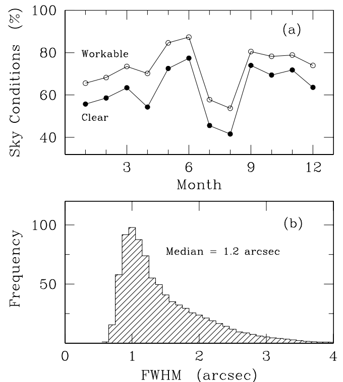
FIG. 2.—Characterizations of the Flagstaff Station observing site, where (a) shows average sky transparency and (b) seeing as a function of calendar date. In (a), “clear” refers to the percentage of clear nighttime hours, while “workable” pertains to conditions with cloud extinctions under 0.75 mag (considered workable with the FASTT). The dip in July and August is caused by the monsoon season in Arizona.
