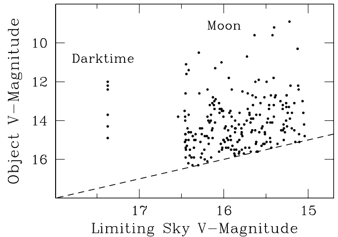
FIG. 7.—The FASTT selects objects for nightly observation according to their brightnesses and the prevailing sky conditions, wherein objects are only picked if the expected S/N of the observation exceeds 7. A model is used to predict the sky brightness that includes the contribution made by the Moon. The figure shows the pick for a night when the Moon rose shortly after nightfall. No objects were chosen below the dashed threshold line, since their images would have been swamped by sky noise. This method of selection is needed in automating observing in order to maximize the number of observations taken in the course of a night.
