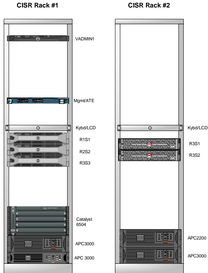
Figure 11. Rack Diagram for the Test Bed.
