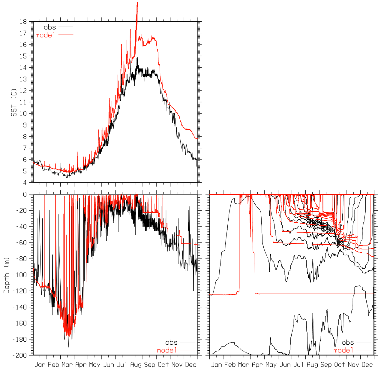
Fig. 6 — SST, MLD, and ISODs at OWS Papa for 1961: observed (black), simulated with the BWS SDC, but without the KC04 LC mixing enhancement (red). ISODs are temporally filtered.
