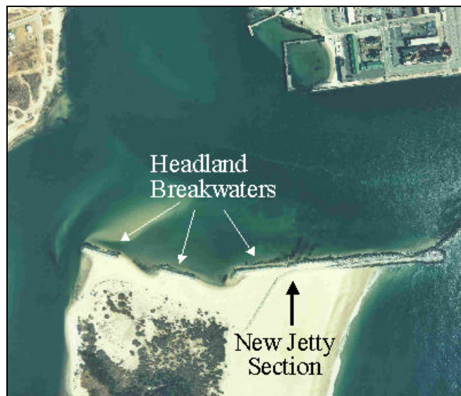
Figure 4c. Ocean City Inlet, Maryland post-project (21 Feb 1990)
