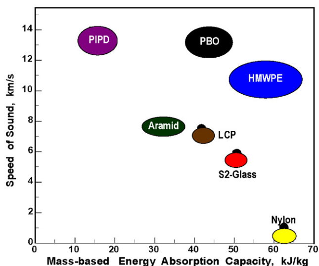
Fig. 1. Sound speed vs. mass-based energy-absorption capacity for a number of high-performance fibers.
