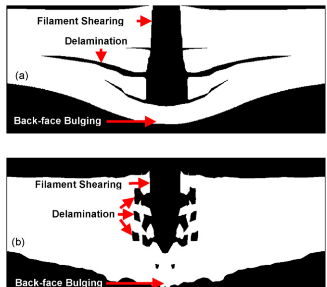
Fig. 7. A comparison between (a schematic of) the experimental results obtained in Ref. [33] (a), and their computational counterparts obtained in the present work (b), pertaining to the spatial distribution of damage in case of a M855 bullet initially propelled at a velocity of 800 m/s impacting a 22-mm thick test panel.
