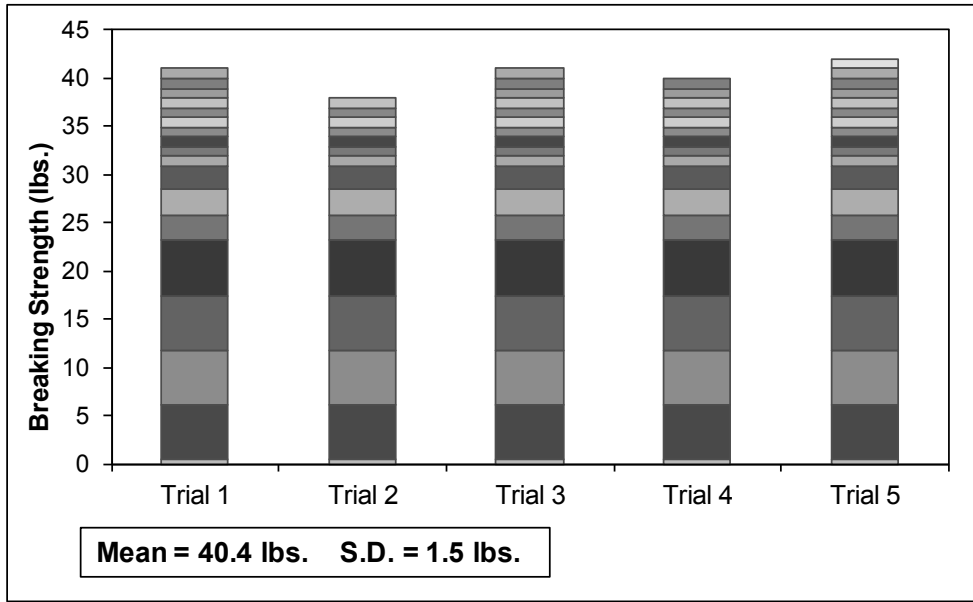
Figure 23. Breaking strength of torpedo guidance wire during the five different trials. Individual bands within a bar represent unique weight increments added during the trial before wire failure.
