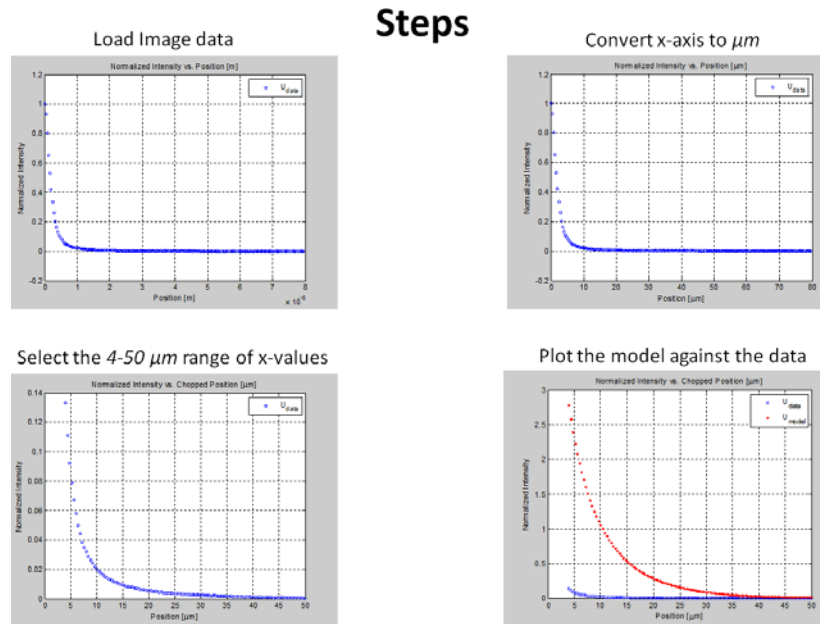
Figure 14. Least square fitting steps showing comparison between the data values (blue) and the mathematical model evaluated at the initial guess values B , L_d , V , and Z_0 .
