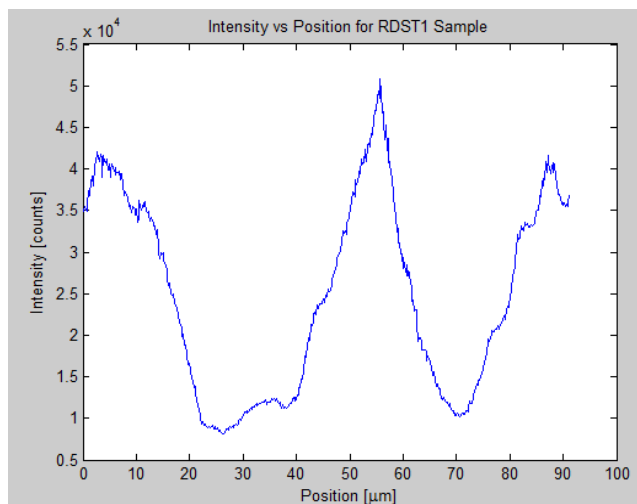
Figure 37. A high-resolution plot of intensity [counts] vs position [μm] suggests that the diameter of the left defect at full width half max is ~20 μm.
