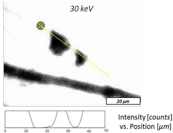
Figure 36. CL image of defects on RDST1 sample at 30 keV at 1500× magnification
