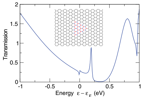
FIG. 14. (Color online) Transmission through a N terminated zigzag edged h-BN nanodomain embedded in graphene (shown as inset) as a function of energy \epsilon relative to the Fermi level \epsilon_F in eV. Note the peak in the transmission at \sim 0.2 eV corresponding to the state localized on the edge of the h-BN nanodomain, shown in Fig. 13(a).
