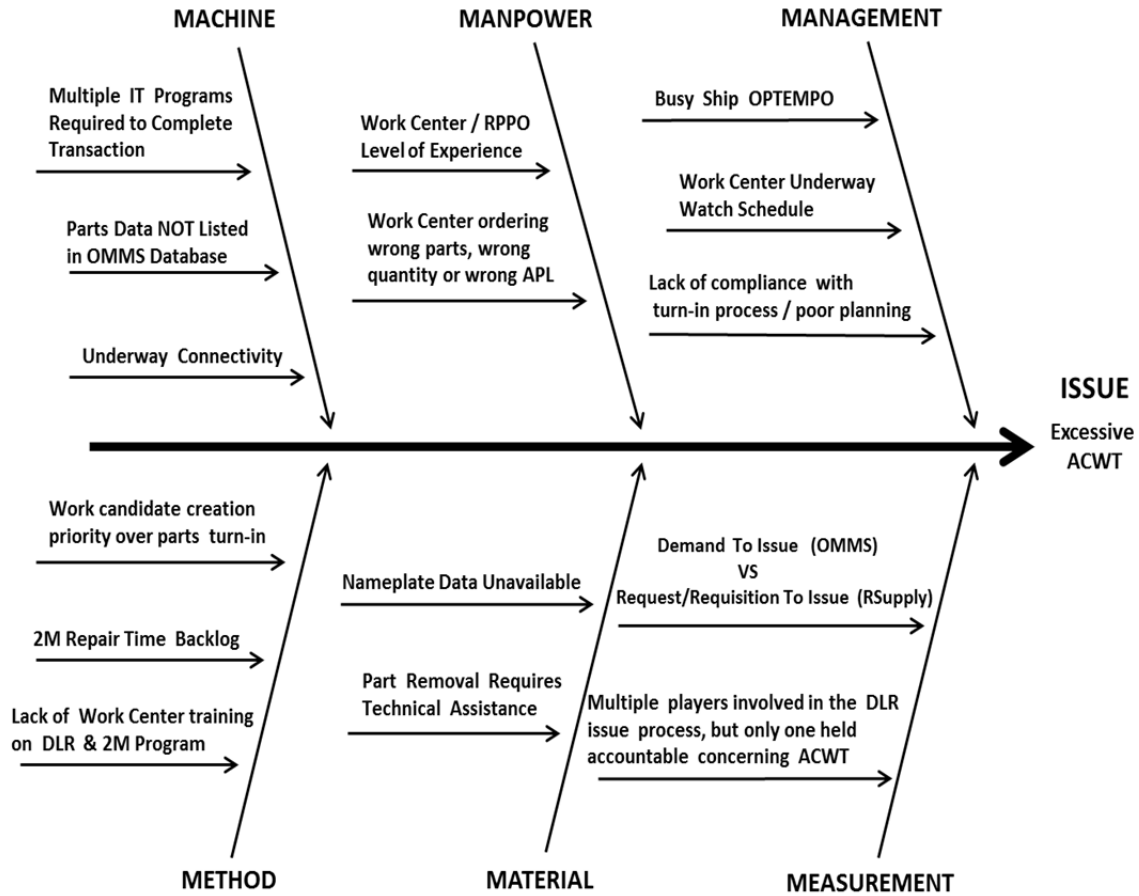
Figure 7. Fishbone Diagram
